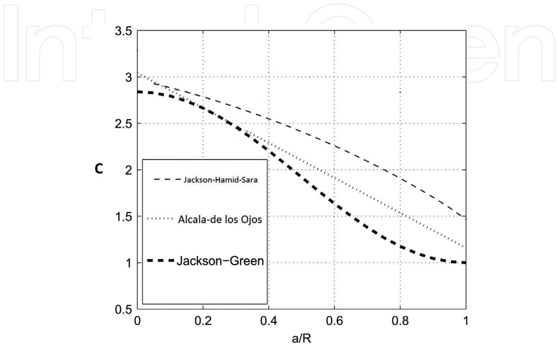
Figure 7. Equations to describe the finite deformation regime for a perfectly plastic material: Jackson-Green [16], Alcalá et al. [17], and Jackson et al. [18] (Adapted from [19]).
