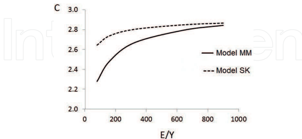
Figure 4. Variation of constraint factor with ratio E/Y following models SK [12] and MM [13], for a material with Poisson's ratio of 0.3.
