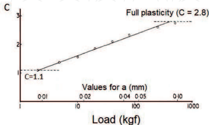
Figure 1. Deformation regimes under sphere-plane contact (Adapted from [5]).
