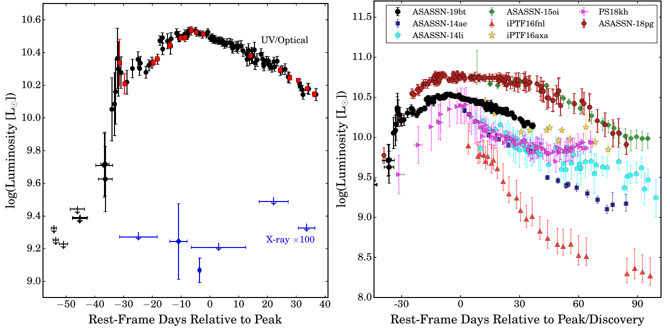
Figure 8. Left panel: evolution of the luminosity of ASASSN-19bt from blackbody fits to the UV/optical Swift sED (red squares) and estimated from the ASAS-SN g-band data by applying bolometric corrections based on the Swift fits (black circles). Swift XRT and XMM-Newton X-ray luminosities are shown as wide and thin blue diamonds, respectively, multiplied by a factor of 100 to improve readability. X-axis error bars indicate data ranges for data combined to obtain a single measurement, and downward arrows indicate upper limits. Right panel: comparison of the luminosity evolution of ASASSN-19bt (black circles) to that of the TDEs ASASSN-14ae (navy squares; Holoien et al. 2014), ASASSN-14li (cyan pentagons; Holoien et al. 2016b), ASASSN-15oi (green diamonds; Holoien et al. 2016a), iPTF16fnl (red triangles; Brown et al. 2018), iPTF16axa (gold stars; Hung et al. 2017), PS18kh (magenta right-facing triangles; Holoien et al. 2018), and ASASSN-18pg (brown hexagons; T. W.-S. Holoien et al. 2019, in preparation). Time is shown in rest-frame days relative to peak for those objects that have observations spanning the peak of the light curve (ASASSN-19bt, ASASSN-18pg, and PS18kh) and in days relative to discovery for those objects that do not (ASASSN-14ae, ASASSN-14li, ASASSN-15oi, and iPTF16fnl).
