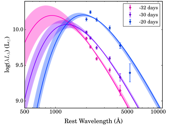
Figure 9. The first three Swift epochs and their blackbody fits. The solid lines show the SEDs of the median luminosity fits to each epoch, and the shaded regions show the range of SEDs for the 16%–84% confidence interval on the luminosity. The phase in rest-frame days relative to peak is given in the legend.
