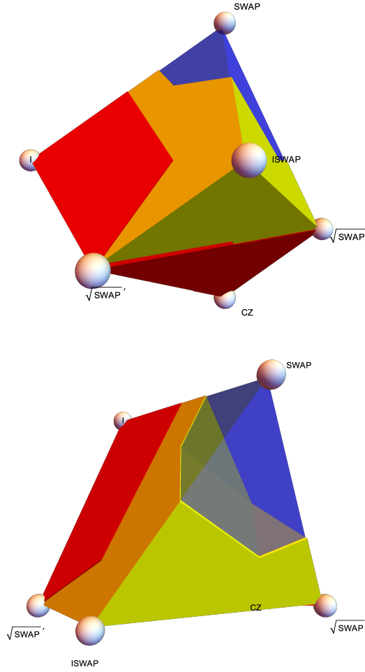
Figure 6: The regions \Pi(P^n_{\sqrt{CZ}}) within \mathfrak{A}_{C_2} : red denotes P^3_{\sqrt{CZ}} , yellow denotes P^4_{\sqrt{CZ}} , and blue denotes P^5_{\sqrt{CZ}} . Not pictured are P^0_{\sqrt{CZ}} and P^1_{\sqrt{CZ}} , each a point, and P^2_{\sqrt{CZ}} , a flat triangle.
