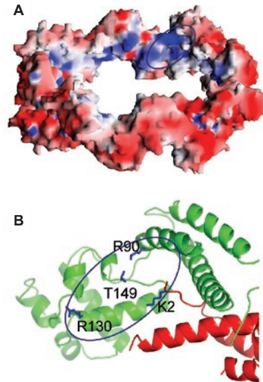
Figure 2. A putative RNA-binding surface inside the ring, which is (A) positively charged and (B) clustered with several conserved residues.
