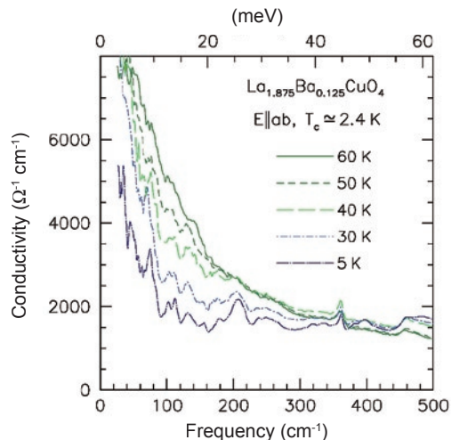
Figure 2. The ab -plane optical conductivity of LBCO for the 1/8 doping in the infrared region between 60 and about 5 K, showing a steady decrease and narrowing of the Drude-like component.
