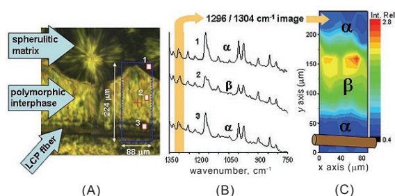
Figure 1. Synchrotron infrared microspectroscopy. (A) Polarized light microscopy of polymorphic iPP interphase, (B) IR spectra recorded through an 8 μm aperture at positions marked, and (C) false-color IR imaging of the interphase region using relative band intensities indicated. The LCP fiber position is also shown.
