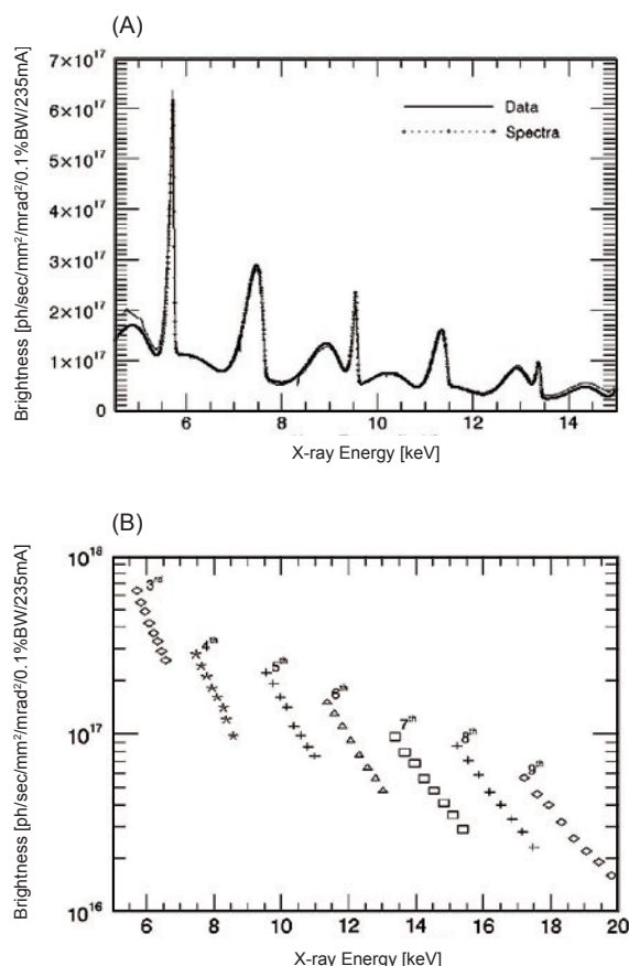
Figure 1. (A) Measured (solid curve) and predicted (dotted curve) brightness spectra of X25 MGU at minimum magnetic gap of 5.6 mm. (B) Measured tuning curves for the 3 rd through 9 th harmonics.
