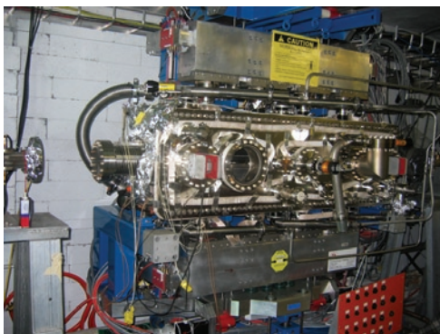
The new X25 MGU installed in the NSLS x-ray ring.
