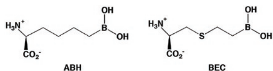
Figure 1. Human arginase inhibitors S-(2-boronethyl)-L-cysteine (BEC, K_d = 270 nM) and 2(S)-amino-6-borohexanoic acid (ABH, K_d = 5.0 nM).
