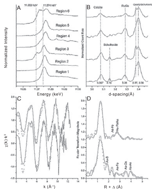
Figure 2. (A) Microfocused XANES spectra at regions 1-6 of selected areas of the As fluorescence maps shown in Figure 1. (B) Microfocused SXRD patterns ( \lambda=0.7598 Å) of As concentrated areas of sample B. Selected diffractograms show 2.8 \text{ Å} < d\text{-spacing} < 3.6 \text{ Å} . (C) Non-linear least-square fits to normalized k^3 -weighted EXAFS spectra of the reference compounds and samples A and B. Raw data and fits are shown by solid lines and open circles, respectively. (D) Non-linear least-square fits to Fourier transforms of the reference compounds and samples A (bottom) and B (top). Raw data and fits are shown in solid lines and open circles, respectively.
