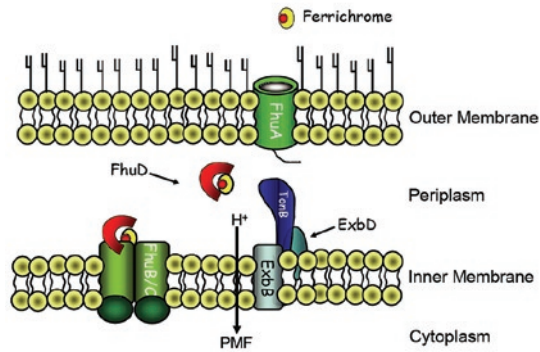
Figure 1. The Ferric Hydroxamate Uptake system (Fhu)
