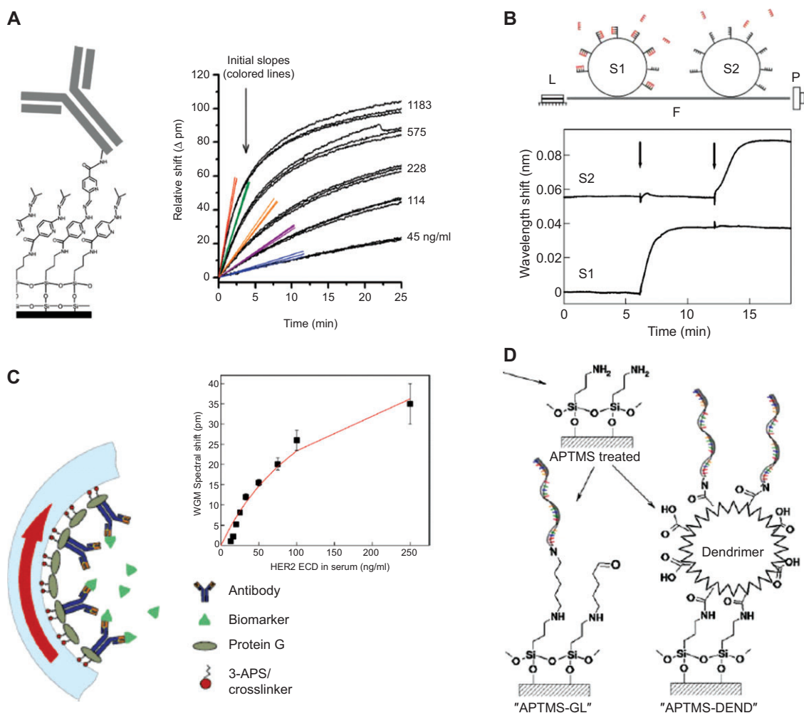
Figure 6 Examples of biorecognition schemes utilized in microresonator biosensing applications: (A) antibody-based detection of a cancer biomarker carcinoembryonic antigen (CEA) with silicon rings in serum (adapted with permission from [85], copyright (2009) American Chemical Society), (B) detection of DNA oligonucleotides by hybridization to dextran-functionalized microspheres (reprinted from [57], copyright (2003), with permission from Elsevier), (C) breast cancer biomarker HER2 detection in LCORRs functionalized with antibody (reprinted from [42], copyright (2010), with permission from Elsevier), (D) silane-based bioconjugation techniques that have been explored for achieving high surface densities in DNA detection [86].
