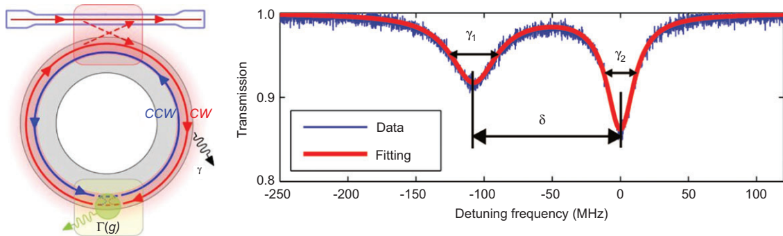
Figure 5 Mode splitting in a WGM resonator. Left: WGM resonators supports degenerate counter-propagating modes: clockwise (CW) and counterclockwise (CCW). Light scattering from a scattering center introduces additional damping to the optical modes and couples the initially degenerate CW and CCW modes, lifting the mode degeneracy. Right: Experimentally obtained mode-splitting transmission spectrum (blue) after the deposition of a single nanoparticle in the mode volume of a microtoroid WGM resonator and the fitted curve (red) adapted from [30].
