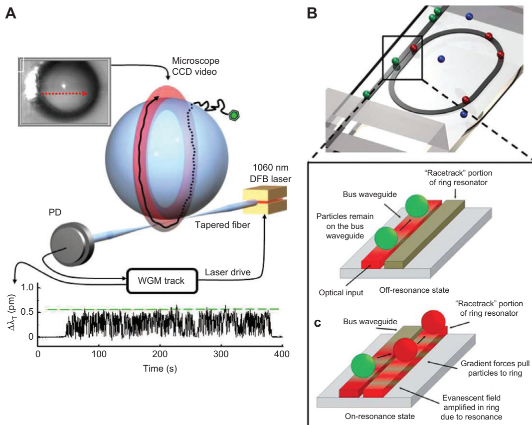
Figure 11 Trapping nanoparticles using gradient force stemming from highly localized field intensities in optical resonators. (A) A nanoparticle is trapped and propelled along the equatorial plane of a fiber taper coupled microsphere, where the fundamental WGM resides, adapted from [32]. (B) A waveguide coupled optofluidic ring resonator is used to manipulate, transport and trap nanoparticles; the particles either pass through the resonator (indicated by particles in green) under off-resonant condition or get trapped on the ring resonator under resonant condition (indicated by particles in red), with permission from [29], reproduced by permission of The Royal Society of Chemistry.
