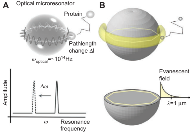
Figure 4 (A) Illustration of a Whispering Gallery Mode (WGM) optical resonance in a glass microsphere. The binding of a protein to the microsphere surface increases the WGM path length by \Delta l , which is detected as a resonance frequency shift \Delta\omega . (B) The reactive sensing principle. A molecule binding to the microsphere surface is polarized within the evanescent field (yellow ring) of a WGM. The energy that is needed to polarize the molecule causes the resonance frequency to shift.
