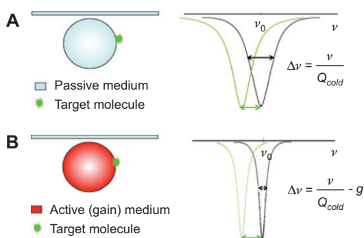
Figure 8 The binding of molecules on the surface of a resonator shifts the resonant frequency. (A) For a passive resonator (resonator without gain medium), too much overlap with the original resonant mode makes it difficult to distinguish the shifted resonance since the resonant frequency shift induced by the attached molecule is smaller than the linewidth. (B) For an active resonator (resonator gain medium), the resonant shift is clearly resolved due to large separation of the shifted resonance from its original position in the spectrum. The narrow linewidth due to the optical gain ( g ) improves the sensor resolution by reducing the smallest detectable shift in the resonance.
