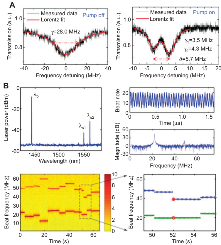
Figure 9 Optical gain to enhance the sensing performance of optical resonators. (A) Typical transmission spectra of an active resonator (resonator doped with optical gain medium) when the excitation pump for the gain medium is off (left: a broad resonance) and on (right: two distinct narrow resonance [70]). (B) Detection of nanoparticles using mode-splitting in a microcavity laser. A beatnote is generated by photo-mixing the split lasing modes in a photoreceiver. The changes in beat frequency with time reflect the scatterer induced frequency splitting in the microlaser which indicates a scatterer entering the laser mode volume. If a multimode microlaser is used, each lasing mode undergoes splitting with the splitting amount depending on the overlap of the scatterer with the volume of the lasing mode. Using a multimode laser reduces the possibility of missing a binding scatterer since one splitting signal could capture a binding event that might have been missed by the other one (lower right panel) adapted from [66].
