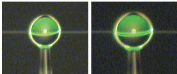
Figure 7 Equatorial WGM. The green ring, which traces the trajectory of the fundamental equatorial WGM, is due to the luminescence of the erbium ions with which the microsphere is doped image taken from [151].
