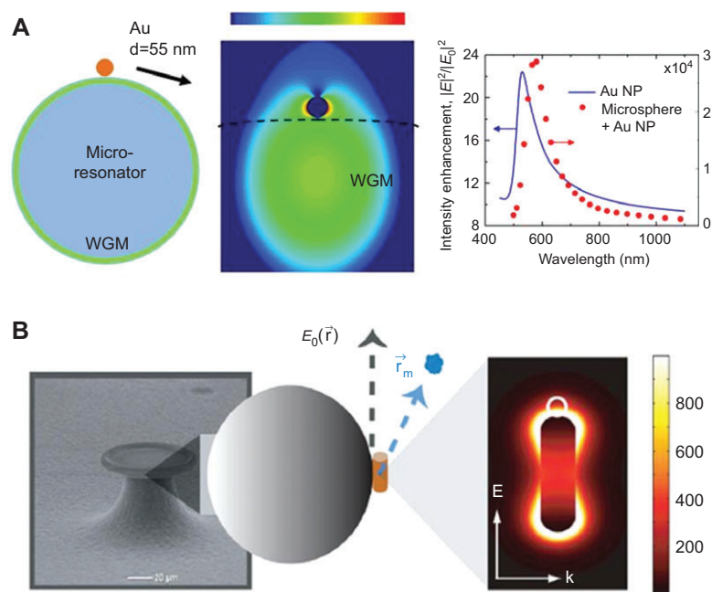
Figure 10 Plasmonic nanoantennas coupled to microcavities enhance sensitivity in biodetection. (A) A molecule binding to a plasmonic nanoantenna coupled to a WGM microcavity experiences field strengths that are enhanced in proportion to E^2/E_0^2 , boosting the frequency shift upon binding [147]. (B) Up to three orders of sensitivity enhancement has been predicted for protein detection with a nanorod coupled to a toroidal cavity, reprinted with permission from [58], copyright (2011), American Institute of Physics.
