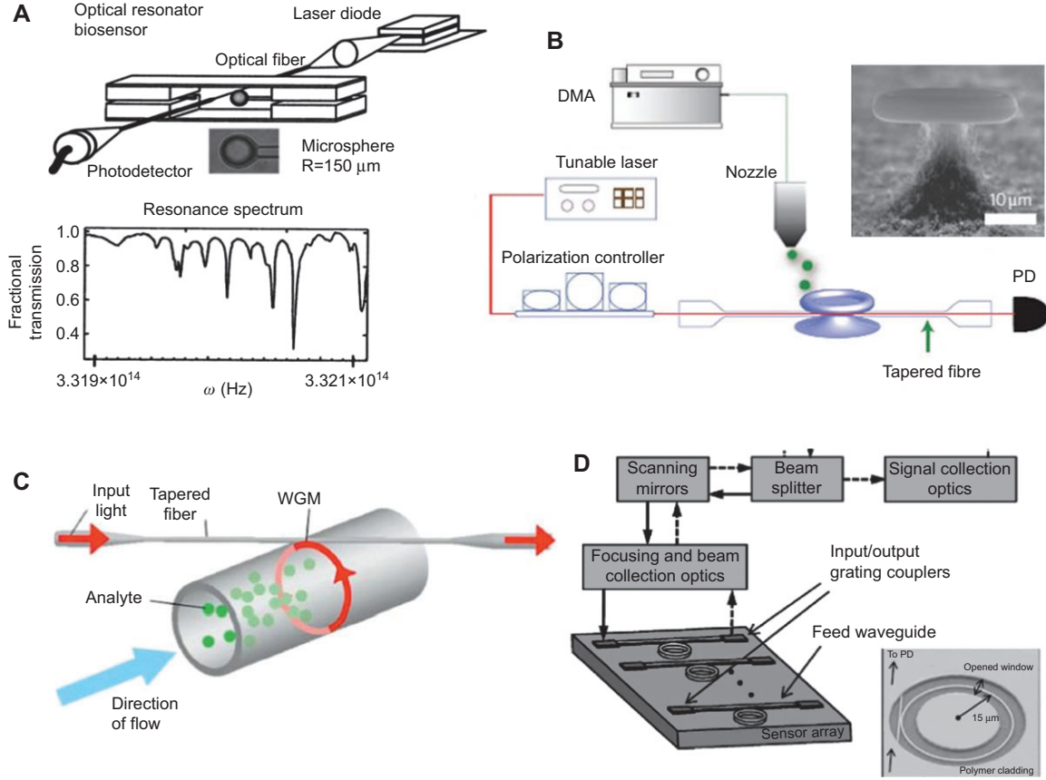
Figure 3 Probing high Q resonances of different optical resonators in biosensor applications. (A–D) Reproduced with permission from [13, 24, 30, 42]. (reprinted with permission from [23]. Copyright (2002), American Institute of Physics. Reprinted from [42]. Copyright (2010), with permission from Elsevier.).
