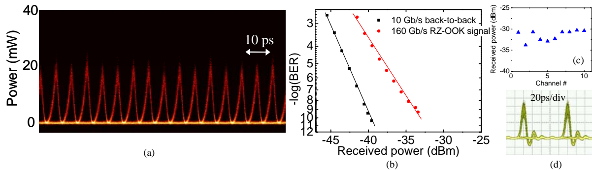
Fig. 4. (a) Optical sampling oscilloscope (OSO) eyediagram of the optically modulated 160 Gb/s RZ-OOK signal; (b) BER measurements for the 10 Gb/s back-to-back RZ-OOK signal and for the optically modulated 160 Gb/s RZ-OOK signal; (c) Receiver sensitivity at the BER of 10^{-9} for the adjacent channels; (d) Eyediagram of the demultiplexed 10 Gb/s RZ-OOK signal from the 160 Gb/s RZ-OOK signal.
