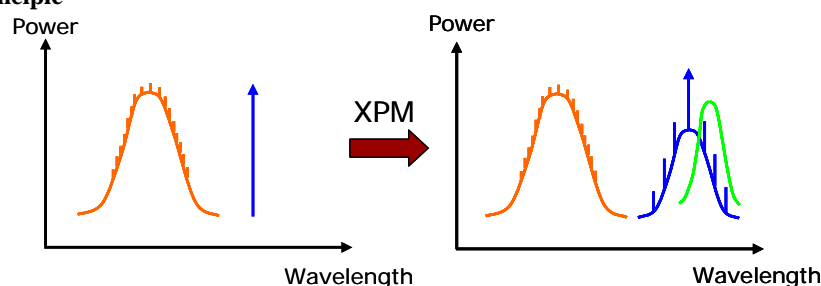
Fig. 1. Schematic of the XPM based all optical modulation with subsequent off-center filtering.
