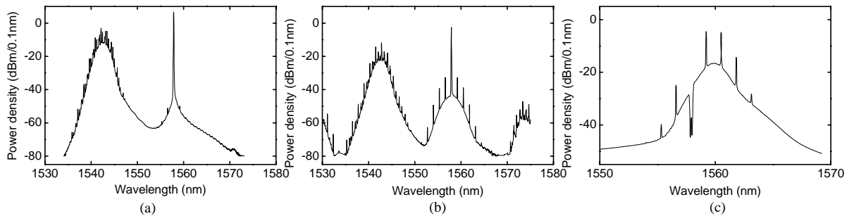
Fig. 3. (a) Spectrum at the input of the silicon nanowire; (b) Spectrum at the output of the silicon nanowire; (c) Spectrum of the modulated 160 Gb/s RZ-OOK signal after the off-center filtering and the carrier suppression.
