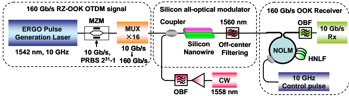
Fig. 2. Experimental setup of 160 Gb/s all-optical data modulation using a silicon nanowire.
