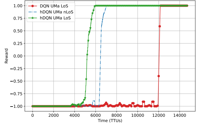
Figure 4: hDQN, DQN training convergence for (N_{TX}, BN_{RX}, N_{RX}) = (2 \times 2, 4 \times 4, 8 \times 8) UPA configuration.
