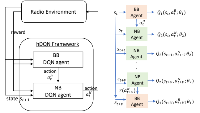
Figure 3: hDQN framework with BB and NB DQN agents
