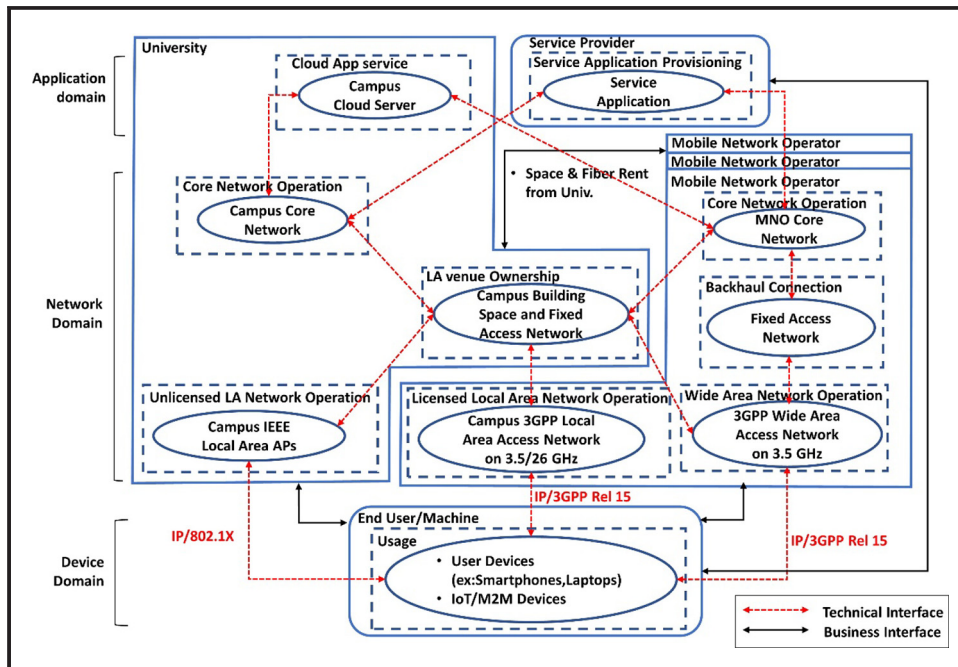
Figure 8 Multi-MNO-driven VNC
