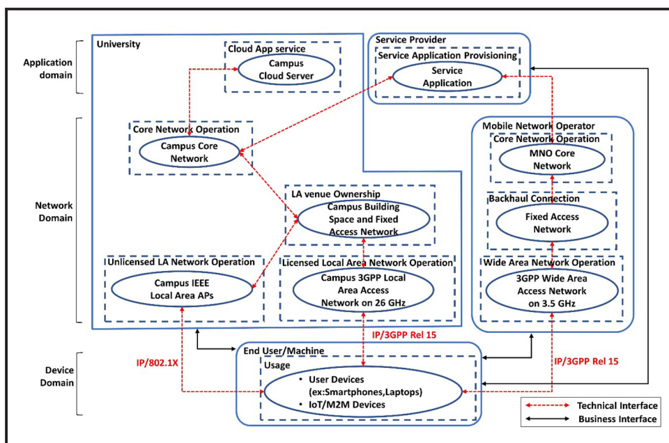
Figure 6 University-driven VNC
