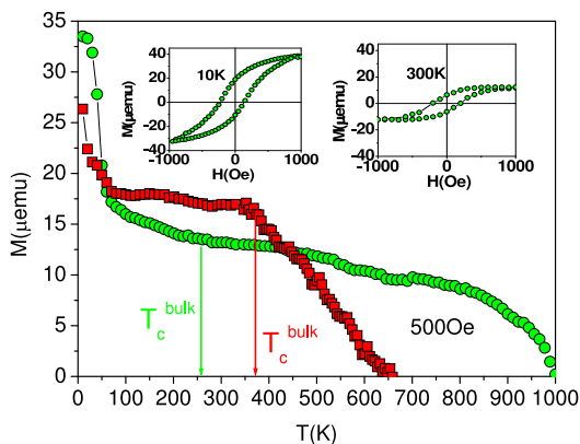
FIG. 4: (Color Online) Magnetization (500 Oerstedes) for the [(\text{La}_{2/3}\text{Sr}_{1/3}\text{MnO}_3)_3(\text{BaTiO}_3)_3]_{25} (red squares) and [(\text{La}_{2/3}\text{Ca}_{1/3}\text{MnO}_3)_4(\text{BaTiO}_3)_4]_{20} (green circles) super-lattices. Hysteresis loops of the calcium super-lattice, recorded at 10 K and 300 K, are presented in the inserts. The arrows mark the bulk Curie temperatures. The surface of both samples is 16\text{mm}^2 .
