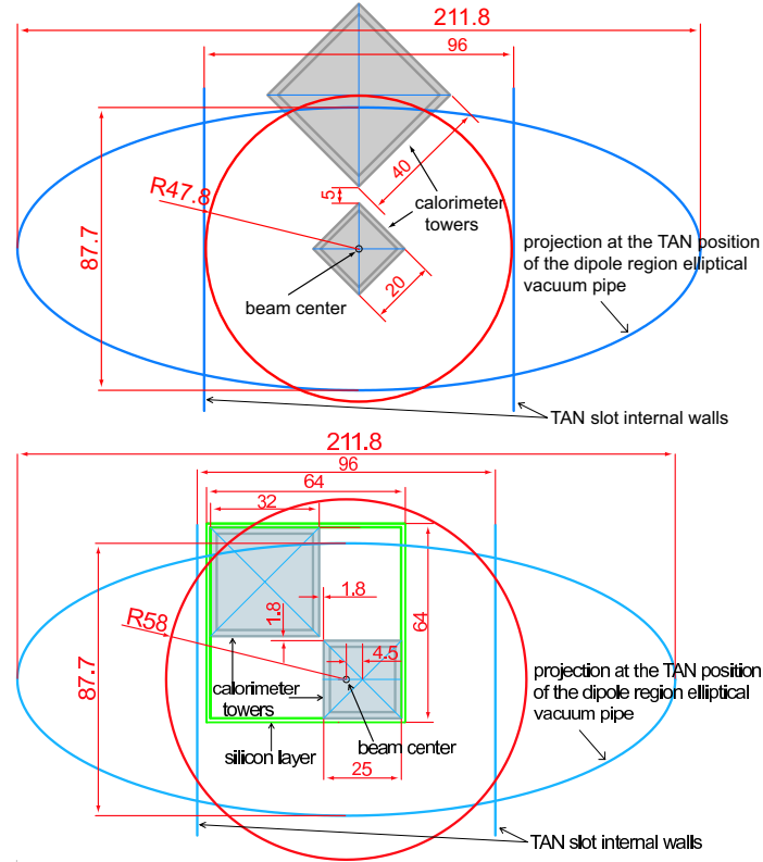
Figure 1.4: Cross sections of detector 1 (top) and detector 2 (bottom). Grey squares indicate the calorimeters in the detectors while a green square shows the coverage of the silicon strip sensor. Vertical and elliptical blue lines indicate the physical aperture limited by the walls of the TAN and the beam pipe, respectively.
