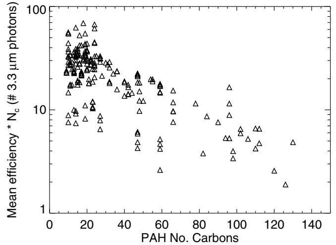
Figure 3. Mean near-IR efficiencies weighted with the solar flux and the cross section, \bar{\epsilon}_i , according to Equation (5), multiplied by the number of carbons as a function of the number of carbons for the neutral PAHs considered in this work.
