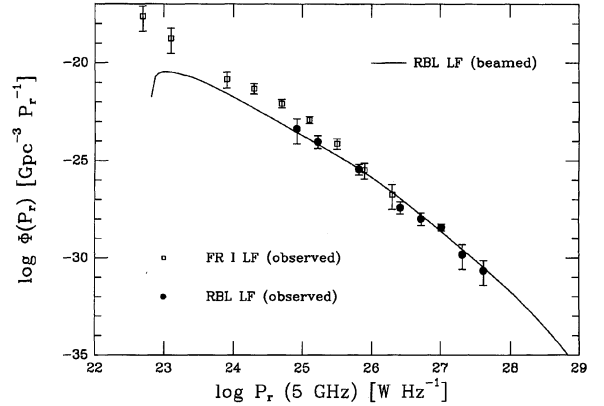
FIG. 17.—The local differential radio luminosity functions of radio-selected BL Lac objects (filled circles; Stickel et al. 1991) and FR I radio galaxies (open squares; Sec. 6.2.4), compared to the fitted beaming model (solid line; first set of RBL parameters in Table 3). Error bars correspond to 1\sigma Poisson errors (Gehrels 1986).
