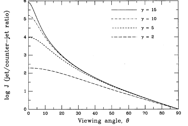
FIG. 22—The jet to counterjet ratio, J , vs. angle to the line of sight for p = 2 . Different curves correspond to different Lorentz factors: from the top down, \gamma = 15, 10, 5, 2 . Note that the ratio is essentially independent of \gamma at large angles.
