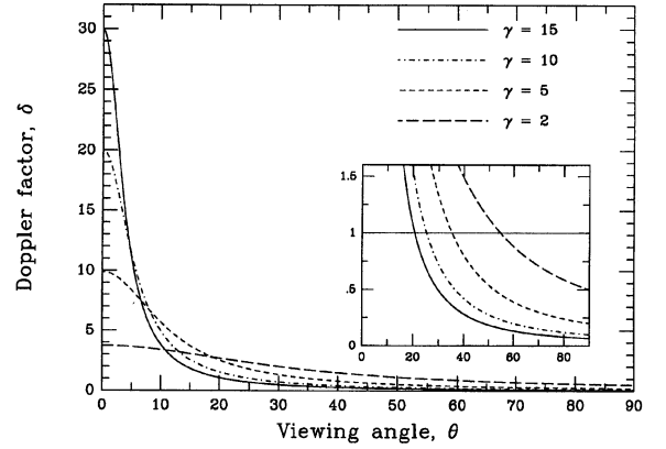
FIG. 20—The dependence of the Doppler factor on the angle to the line of sight. Different curves correspond to different Lorentz factors: from the top down, \gamma = 15, 10, 5, 2 . The expanded scale on the inset shows the angles for which \delta = 1 .
