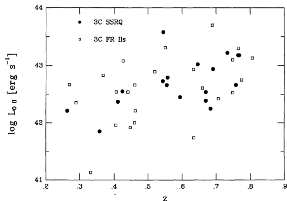
FIG. 7.—The [\text{O II}] emission-line luminosity for quasars (filled circles) and powerful (FR II) radio galaxies (open squares) in the 3CR sample, plotted vs. redshift to allow comparisons at similar radio luminosity (which is well correlated with redshift in a radio-flux-limited sample) and/or observed wavelength of [\text{O II}] . The narrow-emission-line luminosities of radio galaxies and quasars, which should be unaffected by obscuration or relativistic beaming, span the same values over the full redshift range. (Data from Hes et al. 1993.)
