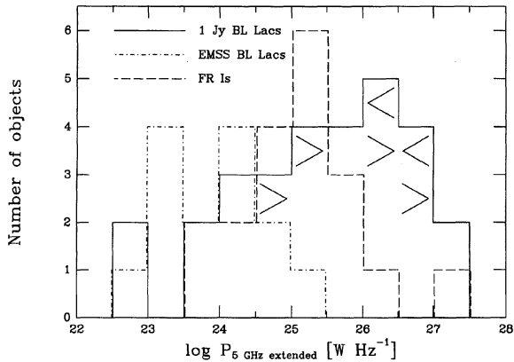
FIG. 10—A comparison of the extended radio powers at 5 GHz for FR I radio galaxies (dashed line) from the 2 Jy sample (Wall and Peacock 1985; di Serego Alighieri et al. 1994b), radio-selected BL Lac objects (solid line) from the 1 Jy sample (Stickel et al. 1991) and X-ray-selected BL Lacs (dot-dashed line) from the EMSS sample (Stoeke et al. 1991). Data for the FR Is come from Morganti et al. (1993); those for RBL have been derived from the R values (Appendix C) given by Padovani (1992a), updated with data from Kollgaard et al. (1992) and Murphy et al. (1993) plus lower limits from Ulvestad et al. (1981); data for the XBL are taken from Perlman and Stoeke (1993). Upper limits on extended power (<) and lower limits on redshift (>) for BL Lac objects are indicated.
