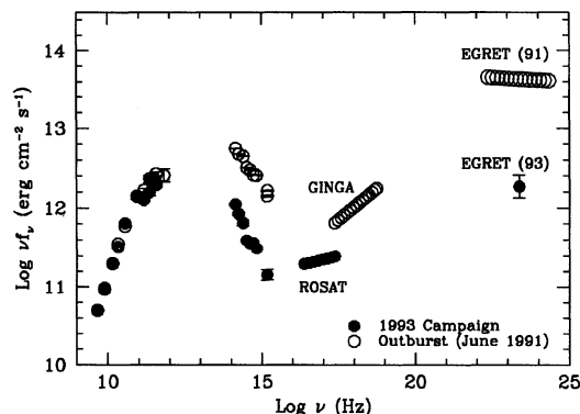
FIG. 4—Multiwavelength spectra of the gamma-ray-bright superluminous quasar 3C279 (Maraschi et al. 1994a) at two epochs, a high state in June 1991 and a low state in January 1993. In the high state, the gamma-ray luminosity is ten times the luminosity in the synchrotron component seen at lower energies, while in the low state the two are comparable. (Copyright American Astronomical Society, reproduced with permission.)
