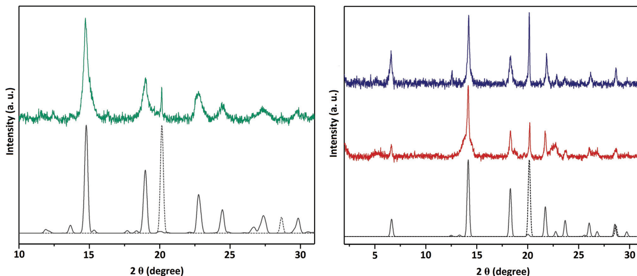
Fig. 3 (Left) X-Ray diffraction patterns of standards for \text{Fe}_{0.48}\text{TiSe}_2 42 (solid black line) and \alpha\text{-iron}^{43} (dashed grey line), and the product of thermolysis at 1000^\circ\text{C} of complex 1 (solid green line); (right) X-ray diffraction patterns of standards for \text{Fe}_{0.16}\text{ZrSe}_2 44 (solid black line) and \alpha\text{-iron}^{43} (dashed grey line), and products of thermolysis at 1000^\circ\text{C} of complex 2 (solid red line) and complex 3 (solid blue line). For clarity, the displayed data are background-subtracted to remove the large contribution from Fe fluorescence.
