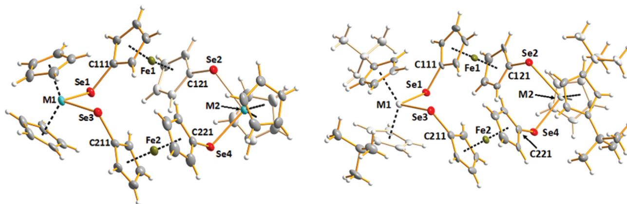
Fig. 1 Molecular structures of [\text{Fe}(\eta^5\text{-C}_5\text{H}_4\text{Se})_2\text{M}(\eta^5\text{-C}_5\text{H}_5)_2] [ \text{M} = \text{Ti} ( 1 ), \text{Zr} ( 2 ), \text{Hf} ( 3 )] (left) and [\text{Fe}(\eta^5\text{-C}_5\text{H}_4\text{Se})_2\text{Hf}(\eta^5\text{-C}_5\text{H}_4t\text{-Bu})_2] ( 5 ) (right) including the numbering of central atoms. Thermal ellipsoids are displayed at a 50% probability level.
