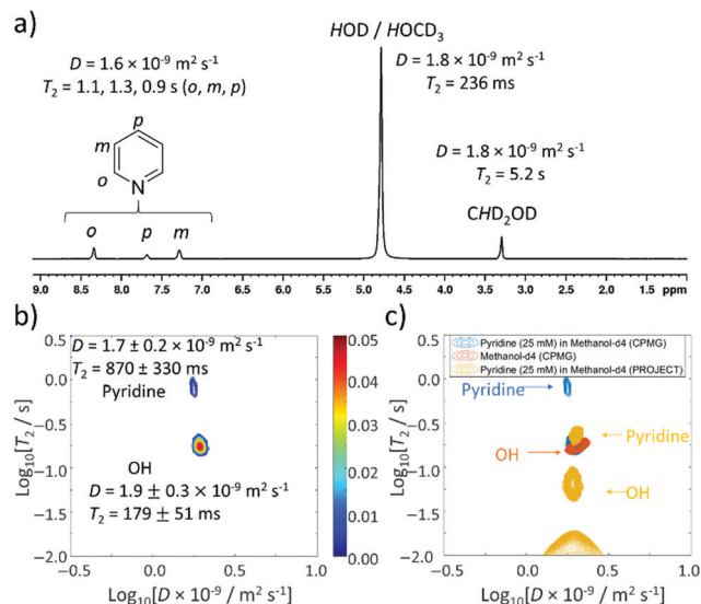
Fig. 4 Thermally polarised ultrafast Laplace NMR of 25 mM pyridine provides a 6.5-fold time saving compared to conventional NMR. (a) ^1\text{H} NMR spectrum with D and T_2 values determined from 1D DOSY and CPMG experiments (36 min each), respectively (b) D - T_2 correlation (with CPMG loop, 11 min) of pyridine (25 mM) in methanol- d_4 (c) D - T_2 correlation plot from (b) (blue) overlaid with that recorded using a PROJECT loop (yellow). A reference sample containing only methanol- d_4 (0.6 mL) recorded using a CPMG loop is also shown (orange). Additional spectra are presented in the ESI† Fig. S2.
