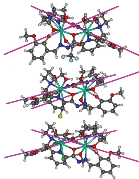
Fig. 8 The principal magnetic axes of the ground Kramers doublets of the two \text{Dy}^{\text{III}} ions in 1 (top), 2 (middle) and 3 (bottom).
