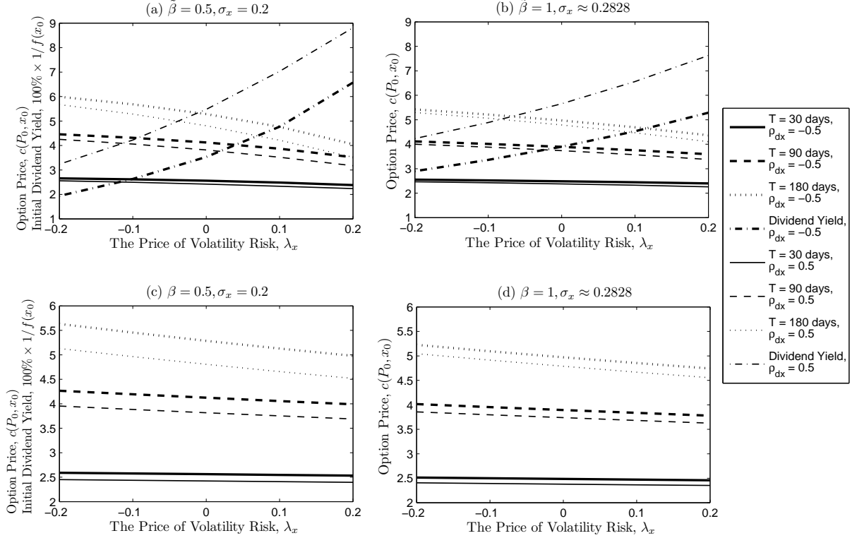
Figure 5: Effect of the price of volatility risk on European call option prices. Parameters are \gamma = 2 , r = 0.02 , \alpha = 0.05 , and \rho_{dx} = -0.5 (thicker lines) or \rho_{dx} = 0.5 (thinner lines). In plot(a) \tilde{\beta} = 0.5 , \sigma_x = 0.2 and in (c), \beta = 0.5 , \sigma_x = 0.2 , and in plots (b) \tilde{\beta} = 1 , \sigma_x \approx 0.2828 and (d), \beta = 1 , \sigma_x \approx 0.2828 . On the other hand, in (a) and (b), \tilde{\beta} is fixed whereas in (c) and (d), \beta is fixed (remember that \lambda_x = \tilde{\beta} - \beta ). Moreover, x_0 = 0.2 , P_0 = \$100 , K = \$100 , and \Delta t = 1/252 year.
