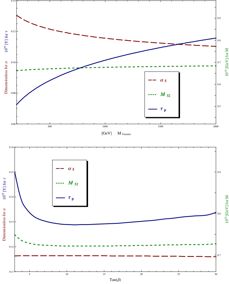
Figure 4: The left-hand numerical scales here perform double duty, read dimensionlessly for \alpha_5 , and in units of [10^{35} \text{ Y}] for the proton partial lifetime \tau_p^{(e\mu^+\pi^0)} . M_{32} is read on the right-hand scale in [10^{16} \text{ GeV}] . The first example visually explores variation of these parameters with respect to changes in the mass of the F-theory vector-like multiplets of Flipped SU(5) Type II. The vector mass is run from 200 [GeV] up to 2 [TeV], bookending the value of 1 [TeV] to which we otherwise default. The SUSY spectrum is taken at benchmark B' as usual. We see a decline in the coupling strength as the vector mass increases, with the (partial) unification mass holding essentially steady. The result is a modest gradual rise in proton lifetime from left to right, starting some 25% below, and ending some 15% above our baseline value. In the second plot we instead vary the SUSY Higgs parameter \tan\beta from 3 to 30, bounding again our default value of 10 for benchmark B'. We regenerate the SUSY spectrum along this span with ISASUGRA, otherwise leaving the B' input parameters intact. This change of approach with respect to the spectrum is responsible for some overall up-tick in the lifetime. The model again is Flipped SU(5) Type II, with the vector mass locked at 1 [TeV]. In this example we instead see \alpha_5 flatline, while the unification mass declines steeply to a minimum near our default region, thereafter rebounding slowly. The proton lifetime tracks with and amplifies changes in the unification mass, although the overall variation is still mild, the peak within about 15% of the valley for the range considered. The slope approaching the left edge however is steep, and continuing too far outside the graph in either direction we experience pathologies in application of the Yukawa boundary condition for calculation of the second loop.
