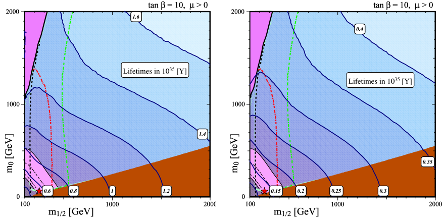
Figure 5: Proton \tau_p^{(e\mu)^+\pi^0} lifetime contours (dark blue), for Flipped SU(5) first with only MSSM field content, and subsequently including Type II vector-like multiplets, are overlaid onto a background map of phenomenological limits on the CMSSM for \tan\beta = 10 , and \mu > 0 , that courtesy of Olive et al. [68]. The orange-brown regions in the lower right of each graphic suffer a charged LSP, while the dark pink at upper left fail electroweak symmetry breaking. The dotted green, red and black lines mark the scalar neutralino-nucleon cross section at 10^{-9} [pB], the Higgs at 114 [GeV], and a chargino mass of 104 [GeV]. The light pink band in the lower left is consistent with measurements of (g-2)_\mu , and the narrow turquoise strip marks agreement between the cosmological CDM limits from WMAP and the relic neutralino prediction after coannihilation. Our baseline benchmark B' (red star) sits in the \mathcal{F} -ast lower left corner of each diagram.
