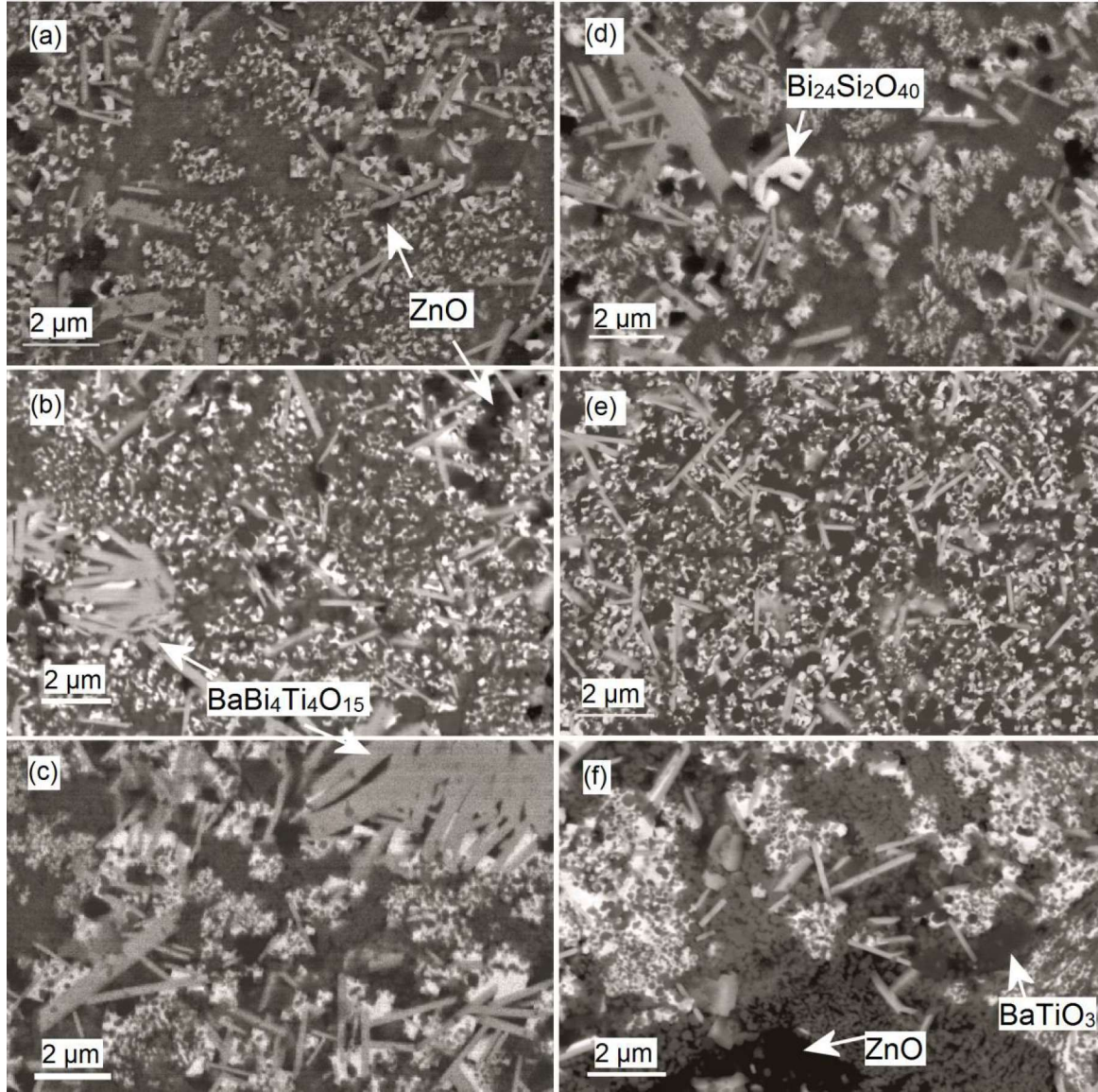
Fig. 6 (a) backscattered electron images A50 and (b) of A50c, (c) A50_LiF (d) A50n, (e) A50nc, and (f) A50nc_LiF samples sintered at 720 °C for 5 hours. Black areas represent ZnO, dark gray BaTiO 3 , light gray BaBi 4 Ti 4 O 15 and the bright ones Bi 24 Si 2 O 40 .
