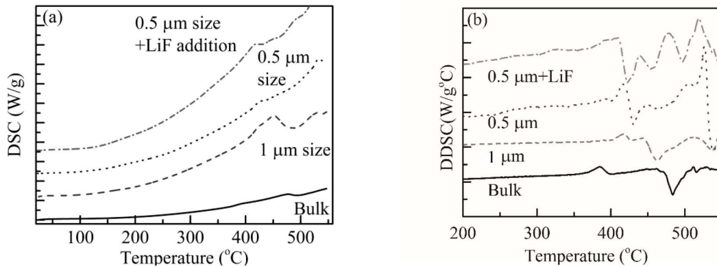
Fig. 2 (a) DSC and (b) differential curves of BBSZ glass with different particle size and LiF addition.
