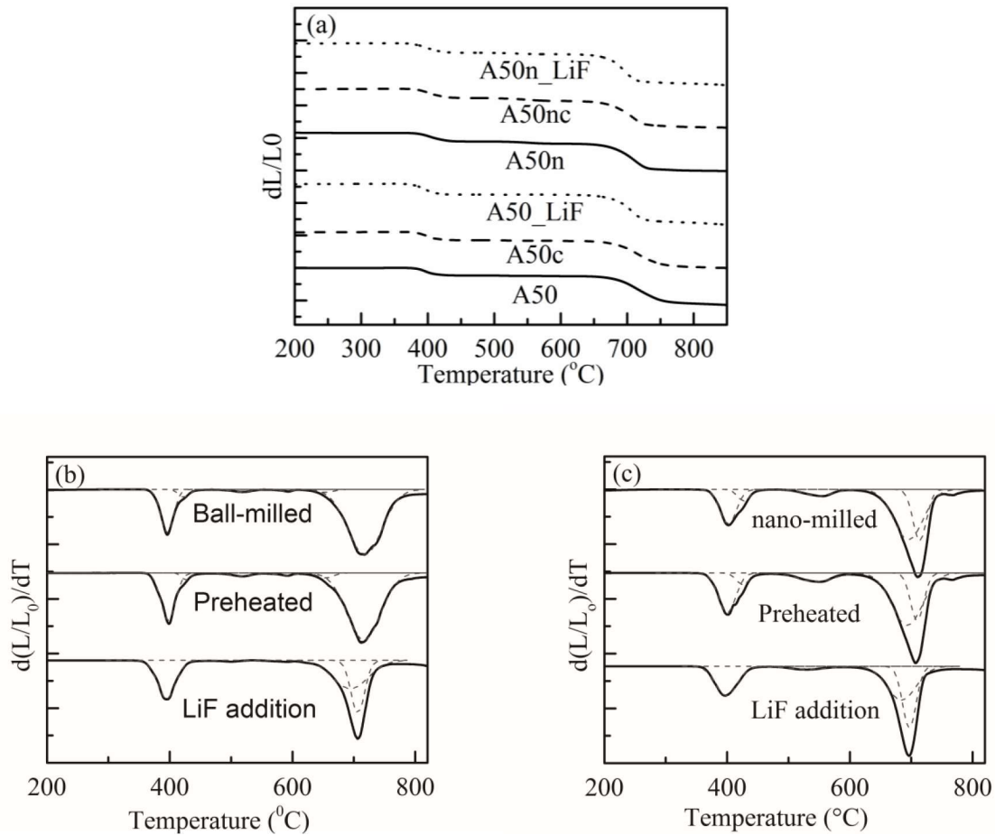
Fig. 3 (a) Dilatometric curves of 50BaTiO 3 -50 wt% BBSZ glass composite with different procedure, (b) and their derivation which were analyzed by Gaussian peaks.
