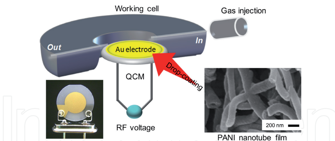
Figure 5. Schematic representation of the interaction of an analyte with PANI nanotube prepared with CSA coating on a QCM (modified and adapted with permission from Ref. [194]. Copyright 2014, Wiley-VCH Verlag GmbH & Co. KGaA, Weinheim).
