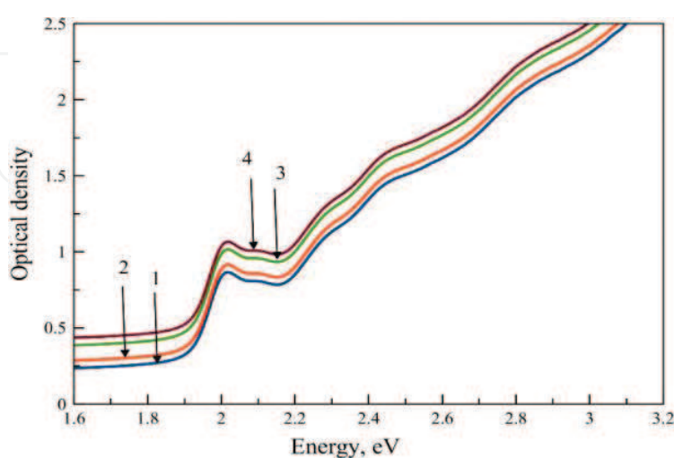
Figure 11. Absorption spectra of FP glasses doped with CdSe QDs with size of 4.5 nm after laser irradiation at power density 15 mJ during 0 min (1), 5 min (2), 10 min (3) and 15 min (4) at \lambda_{\text{exc}} = 355 nm. The diameter of the laser beam is 4 mm.
