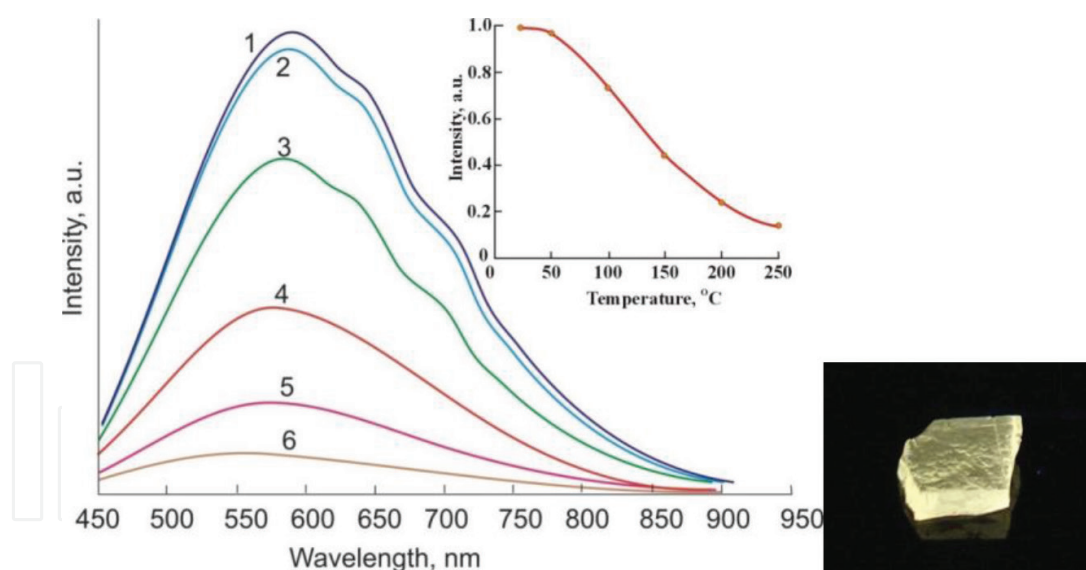
Figure 18. The influence of the temperature of the FP glasses doped with (\text{PbSe})_n MCs on the luminescence intensity... The luminescence spectra were measured at temperature of (1) 22°C, (2) 50°C, (3) 100°C, (4) 150°C, (5) 200°C and (6) 250°C. Excitation wavelength was of 405 nm. Inset: Luminescence intensity in maximum via the temperature of the sample and photo of the luminescence of the FP glass doped with (\text{PbSe})_n MCs.
