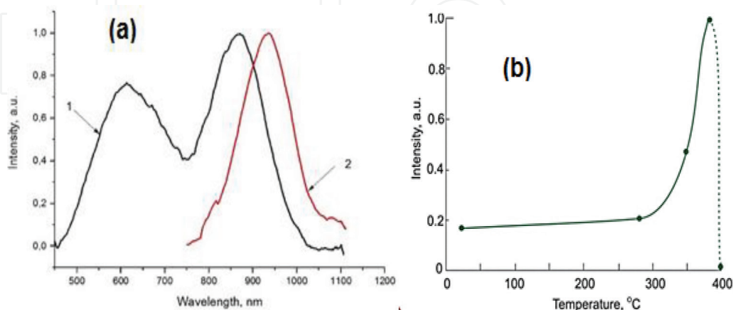
Figure 17. (a) Luminescence spectra of FP glass doped with MCs (\text{PbS})_n after heat treatment at 400^\circ\text{C} within 90 min (1) and 97 min (2), E_{\text{ex}} = 3.06 eV and (b) Luminescence intensity in maximum as a function of thermal treatment temperature.
