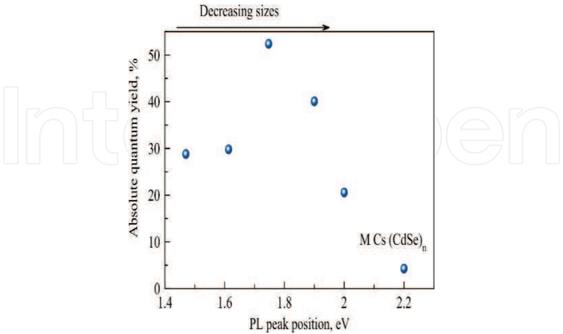
Figure 7. Dependence of the PL AQY on the PL peak position of the CdSe QDs.
