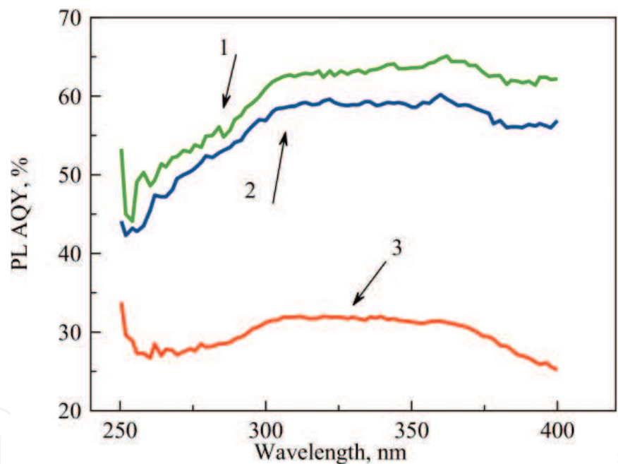
Figure 10. Dependence of PL AQY magnitudes for glasses doped with CdS QDs with sizes 2.3 nm (1), 3.5 nm (2) and 1.8 nm (3), respectively, on the excitation wavelength.
