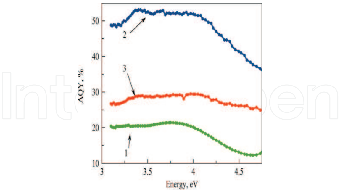
Figure 6. Dependence of the PL AQY for FP glasses doped with CdSe QDs with sizes 2.0 nm (1), 3.0 nm (2) and 4.0 nm (3) on the excitation energy.
