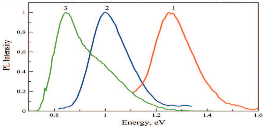
Figure 19. Luminescence spectra of the glasses doped with PbS QDs with sizes 3 nm (1), 3.9 nm (2), 4.9 nm (3) and \lambda_{\text{exc}} = 808 nm.
