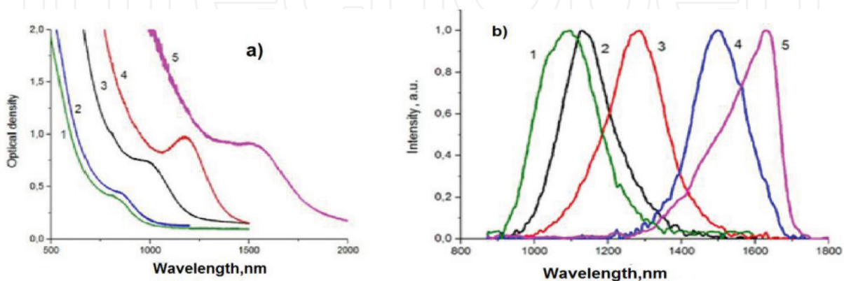
Figure 20. Absorption (a) and luminescence (b) spectra of the glasses doped with PbSe QDs with sizes 2.5 nm (1), 3.0 nm (2), 3.7 nm (4), 5.1 nm (5), \lambda_{\text{exc}} = 808 nm.
