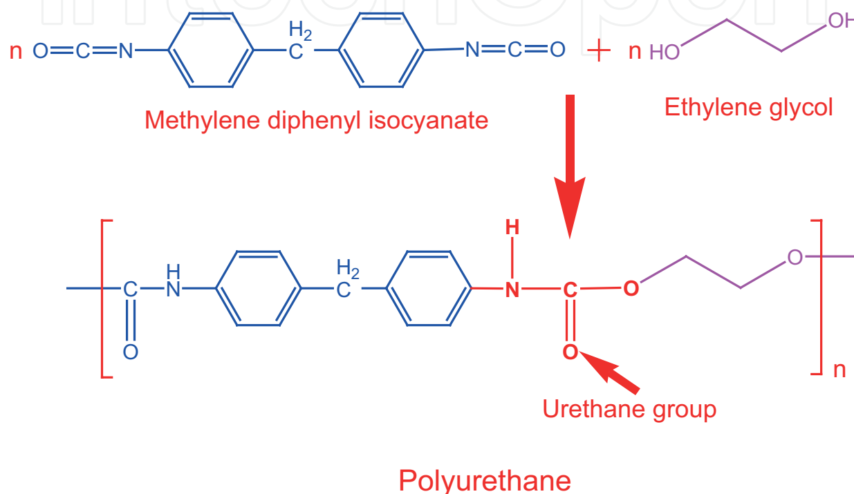
Figure 1. Chemical structure of PU elastomer.
