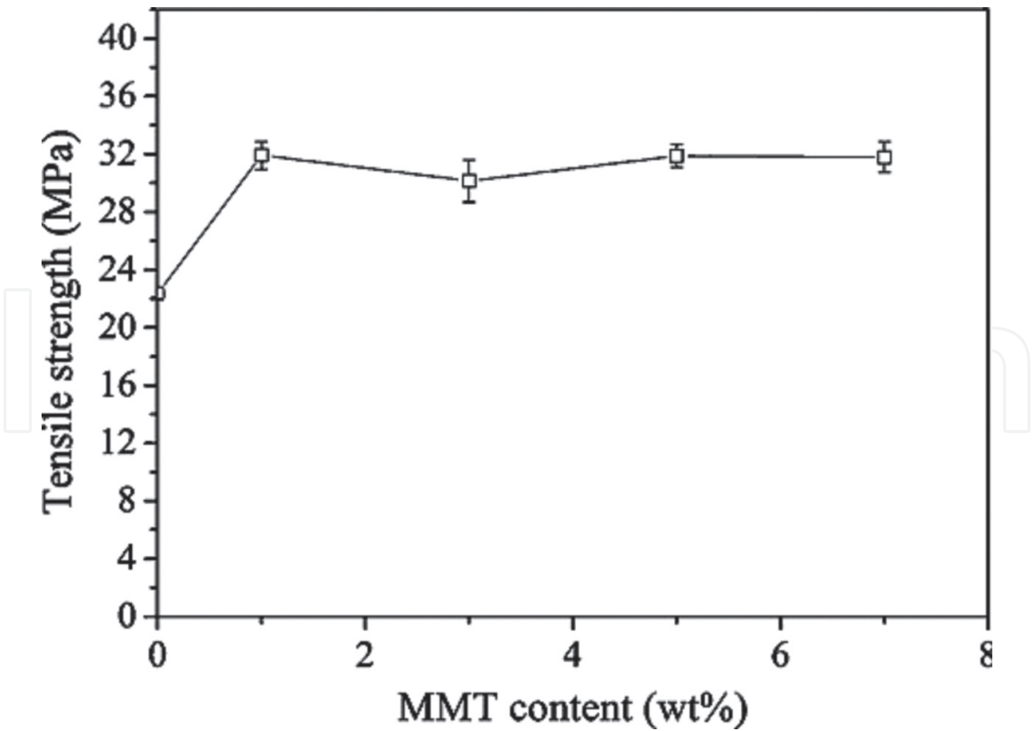
Figure 6. Tensile strength of MMT-filled PU/EP IPN composites as a function of the MMT content [8].
