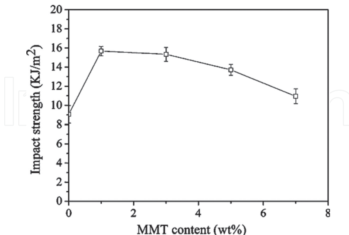
Figure 7. Impact strength of MMT-filled PU/EP IPN composites as a function of the MMT content [8].
