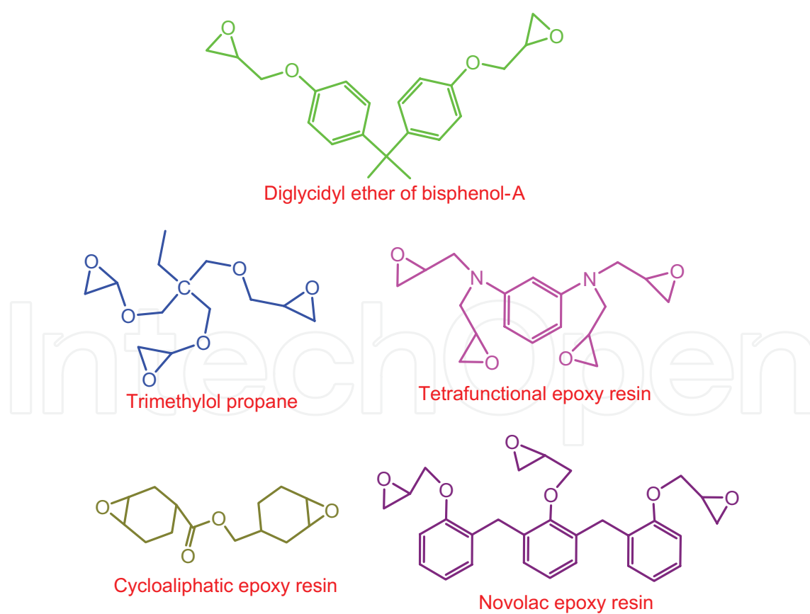
Figure 3. Different types of epoxy resin.
