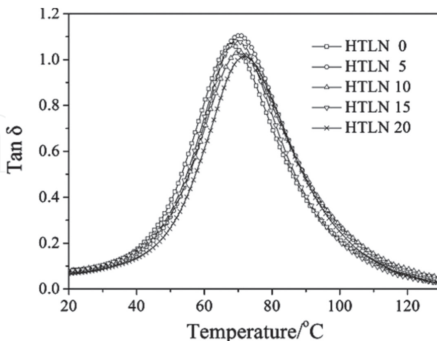
Figure 5. DMA curves of PU/EP IPN composites as a function of the HTLN content at 10 Hz [46].
