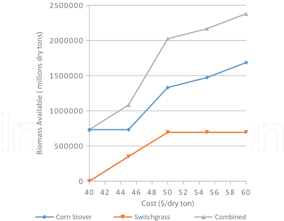
Figure 3. Biomass availability in northwestern Kansas as a function of farmgate price; prices and quantities shown are for 2015 and assume base case yields [34]. Supply curves illustrate biomass availability as a function of cost for a 12-county region in northwestern Kansas, with an approximate area of 90 miles \times 120 miles. Curves are shown for corn stover (blue), switchgrass (red), and combined for a blended supply of corn stover and switchgrass (green).
