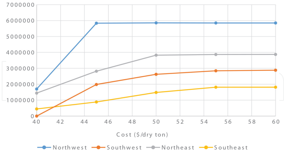
Figure 2. Feedstock supply curves for various locations in Iowa [33]. Availability and cost assume base case corn stover yields for 2015 for 61 counties in Iowa.
