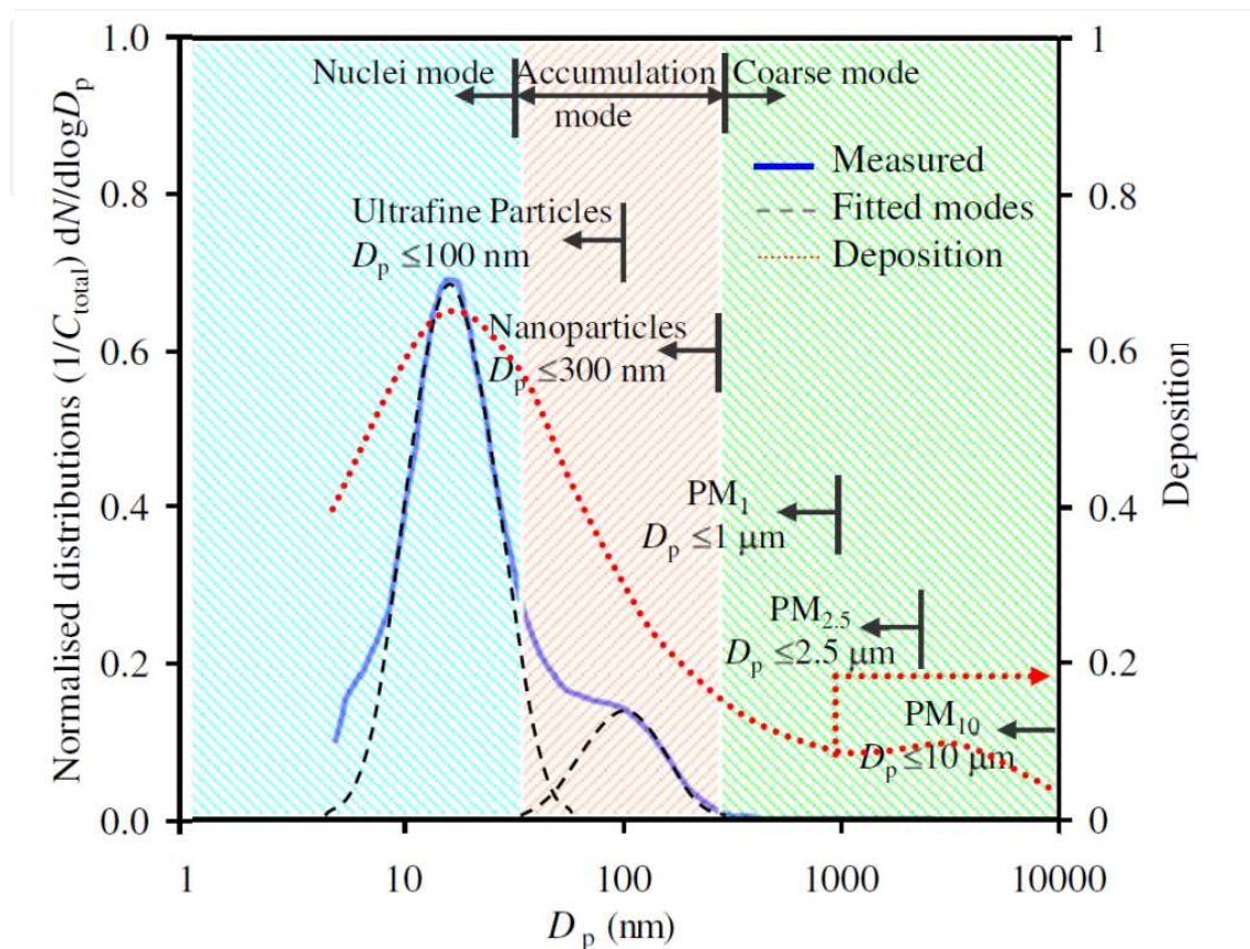
Figure 2. Distribution of atmospheric particles in street canyon in Cambridge, UK (Kumar et al., 2008); D_p is particle diameter. Definitions of atmospheric particles and their size dependent deposition in alveolar and tracheo-bronchial regions are also shown. Adapted from Kumar et al. (2010).
