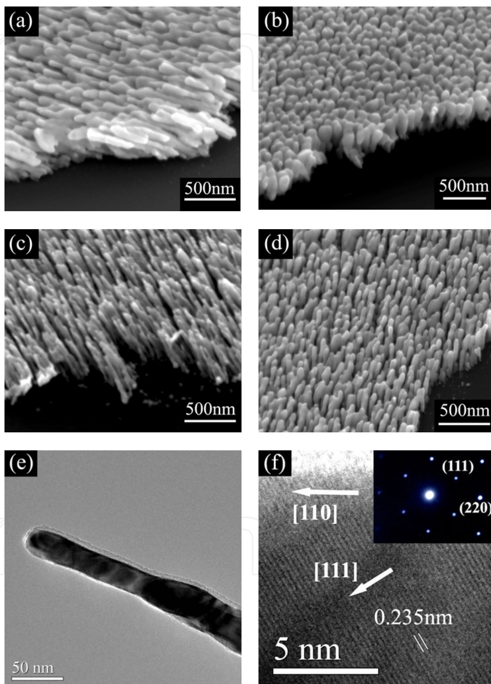
Figure 1. Growth morphology of thin Ag films by GLAD at various conditions. (a) at 120 °C without substrate rotation; (b) at 120 °C and substrate rotation at 0.2 rpm; (c) at -40 °C without substrate rotation; and (d) at -40 °C and substrate rotation at 0.2 rpm. (e) and (f) shows respectively a bright-field TEM and a HRTEM image of the nanorods shown by Fig 1(c); inset of (f) is the corresponding SAD pattern.
