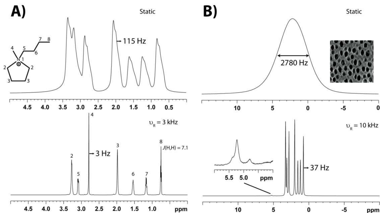
Figure 6. The ^1\text{H} HR-MAS NMR of the ionic liquid [MBPyrr] ^+ [TFSI] ^- at 298K as A) neat liquid and B) adsorbed (20 wt%) into an aluminum oxide ANOPORE inorganic membranes (200 nm pore diameter). The spectra in the top portion of each figure were obtained under static conditions, with the spectra in the bottom portions of each figure obtained under MAS conditions.
