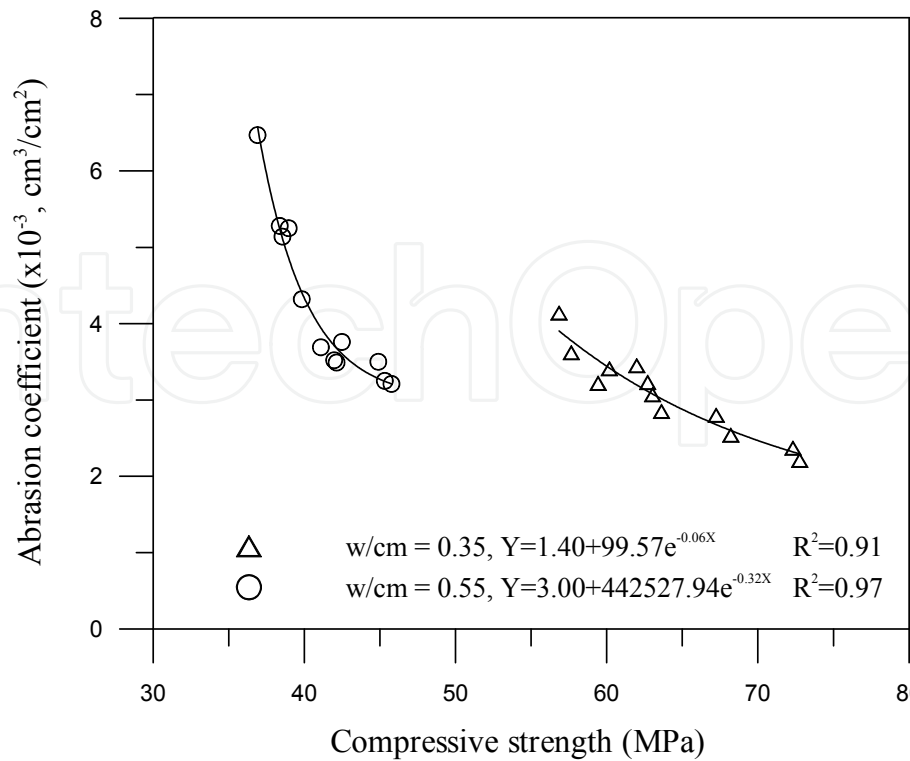
Fig. 3.2. Abrasion coefficient vs. compressive strength curves
