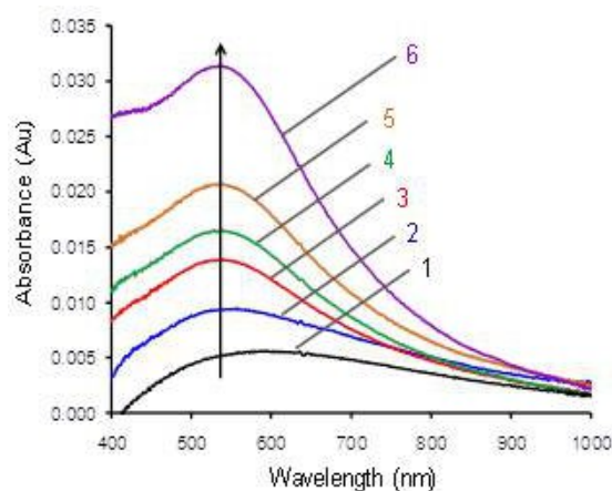
Figure 3 Representative UV-Vis spectral monitoring of a dithiol-linked MPC film growth on a 3-MPTMS modified glass slide. A dip cycle consists of an exposure of the glass slide to NDT linker solution followed an exposure to MPC solution. Each subsequent dip results in growth in film thickness and a concurrent absorbance increase. As the number of dip cycles increases, the surface plasmon band is gradually defined at ~520 nm. Reprinted with permission from M.L. Vargo, C.P. Gulka, J.K. Gerig, C.M. Manieri, J.D. Dattelbaum, C.B. Marks, N.T. Lawrence, M.L. Trawick, and M.C. Leopold, Langmuir 26(1), 560-569. Copyright 2010 American Chemical Society.
