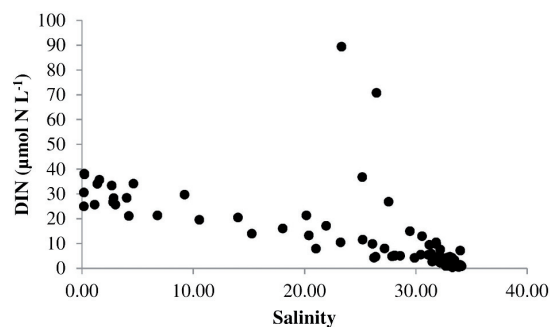
Fig. 10—DIN–salinity curve for the Liffey Estuary representing all data points in 2010. The divergence from the straight line relationship between DIN and salinity is indicative of the influence of the Ringsend WWTP facility at the lower end of the estuary.
