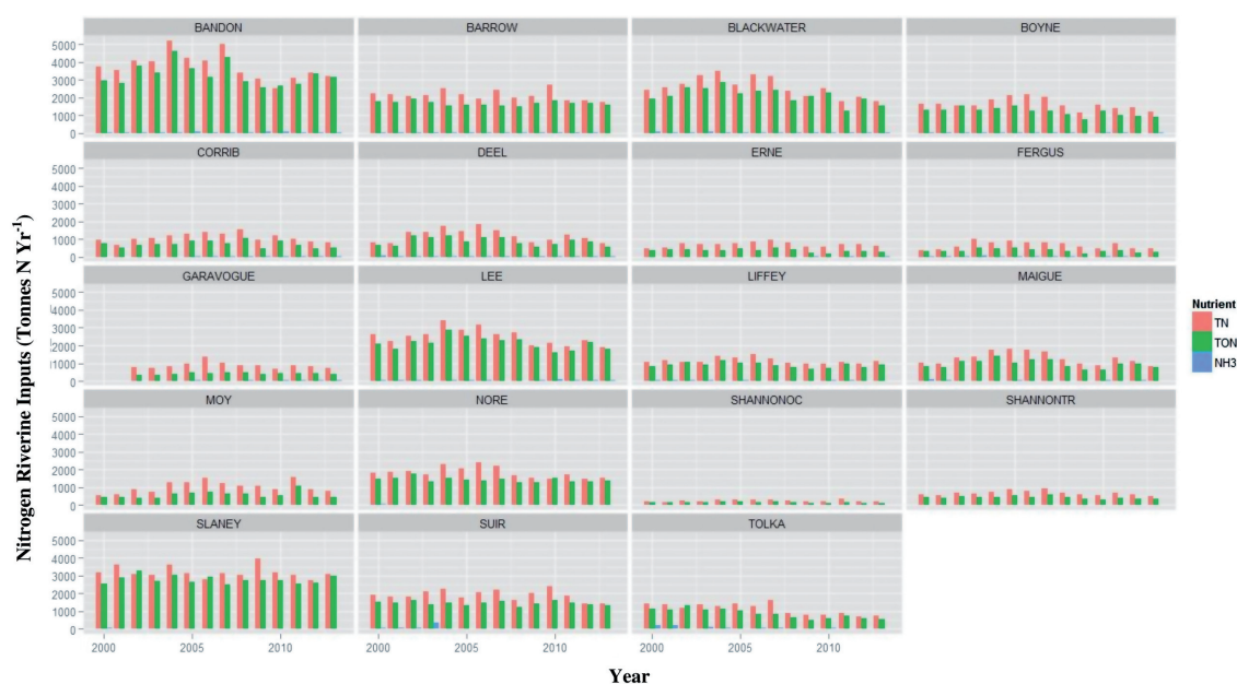
Fig. 6—Annual flow normalised total nitrogen (TN), total oxidised nitrogen (TON) and ammonium ( \text{NH}_3 ) exported downstream from the eighteen riverine systems to transitional and coastal areas between 2000 and 2013.
