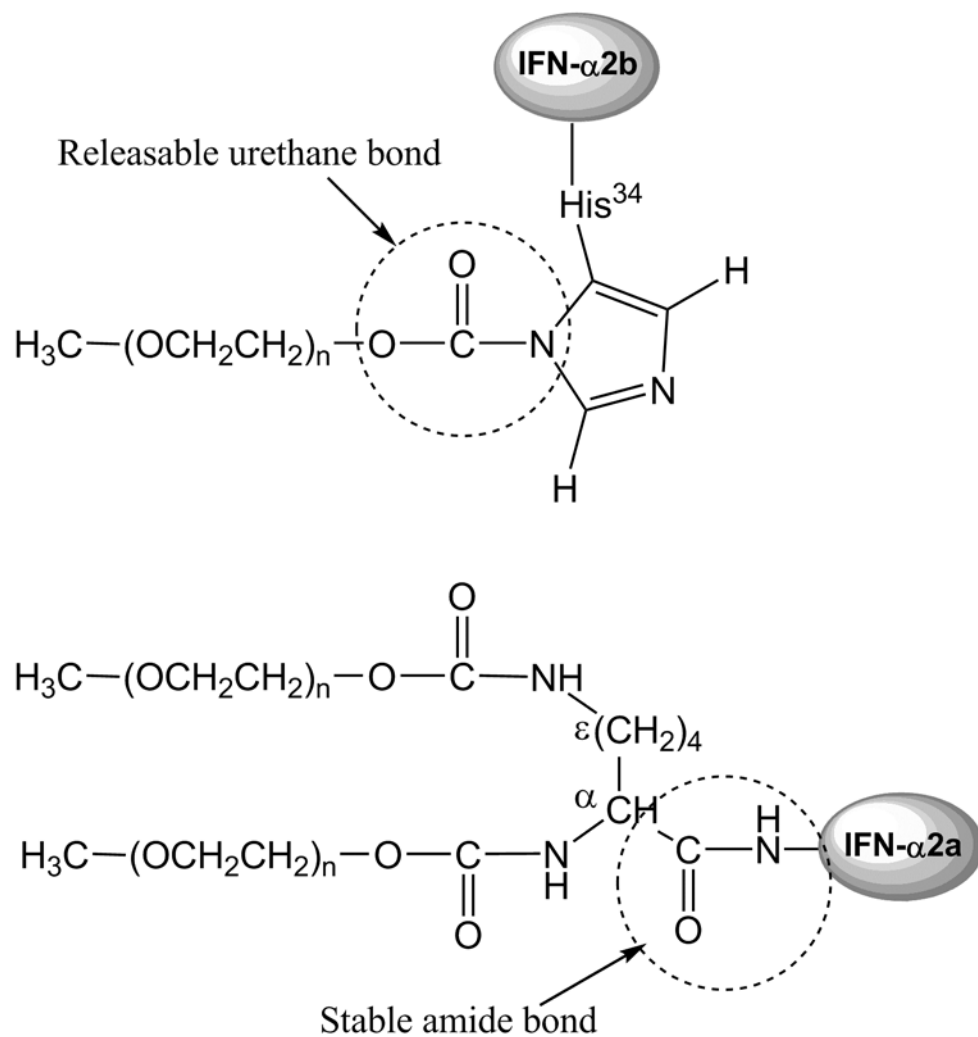
Figure 5. Differences on the PEGylation strategy for PegIntron ® (PEG-IFN-α2b) and Pegasys ® (PEG-IFN-α2a).
