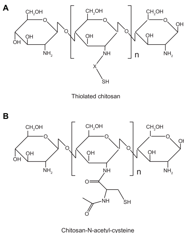
Figure 3 Representative structure of thiolated chitosan: (A) general structure of thiolated chitosan modified by an -SH group ( X : linker) and (B) chitosan-N-acetyl-cysteine (modification of chitosan at the D-glucosamine unit by N-acetyl-cysteine).
