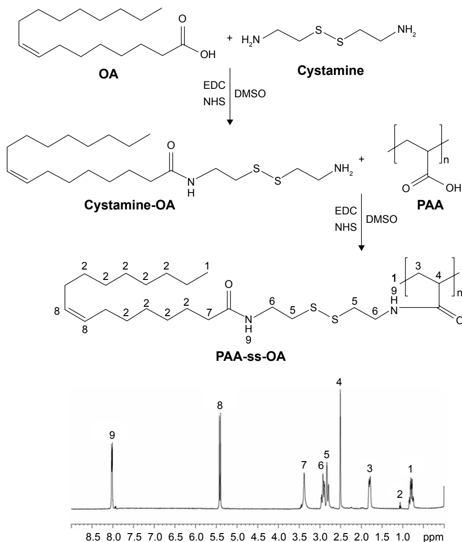
Figure 1 Synthesis route and 1 H-NMR spectroscopy of PAA-ss-OA.
