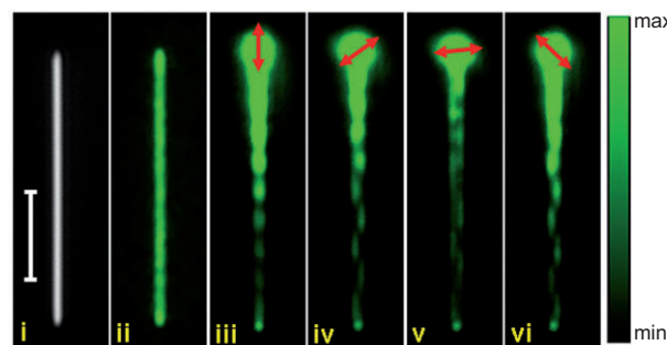
Figure 7 QD emission images of plasmons launched by 632.8 nm laser excitation at one end of a Ag nanowire. Changing the polarization angle at the input modifies the field distribution in the nanowire. (i) Optical image of a Ag nanowire. (ii) The QD emission image with wide field excitation. (iii–vi) QD emission images for different polarizations of the incident laser. The scale bar is 5 \mu\text{m} . The red arrows indicate the laser polarization [77].
