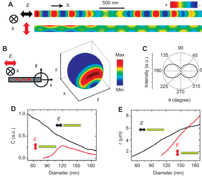
Figure 4 SPP modes in nanowires with flat terminations. (A) Charge distribution on the surface of a wire of the length 3.36 \mu\text{m} and diameter 130 nm, terminated by flat ends. The left end is excited by a 633 nm wavelength focused beam with polarization parallel and perpendicular to the wire, respectively. (B) The resulting spatial distribution of the emission intensity on a sphere enclosing the wire end excited by the parallel incident polarization. Colored and black lines represent the intensity and the polarization of the emission on the sphere. (C) Emission intensity of different polarizations from a wire excited under the parallel polarized excitation. (D) The in-coupling efficiency C for two SPP modes (black curve for m=0 mode, red curve for m=1 mode) as a function of the wire diameter. (E) The 1/e damping length, r , of both modes as a function of the wire diameter [43].
