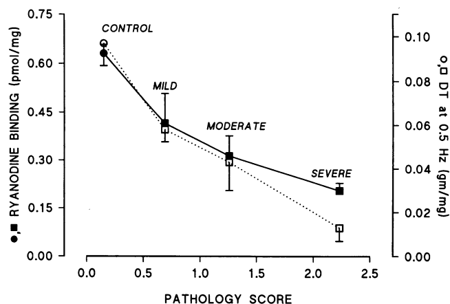
Figure 6. Comparison of ryanodine binding (solid symbols) ( \text{pmol/mg} ) and developed tension ( \text{DT} ) (open symbols) ( \text{g/mg} at 0.5 Hz) as a function of cardiomyopathy severity. Values represent mean \pm SE.
