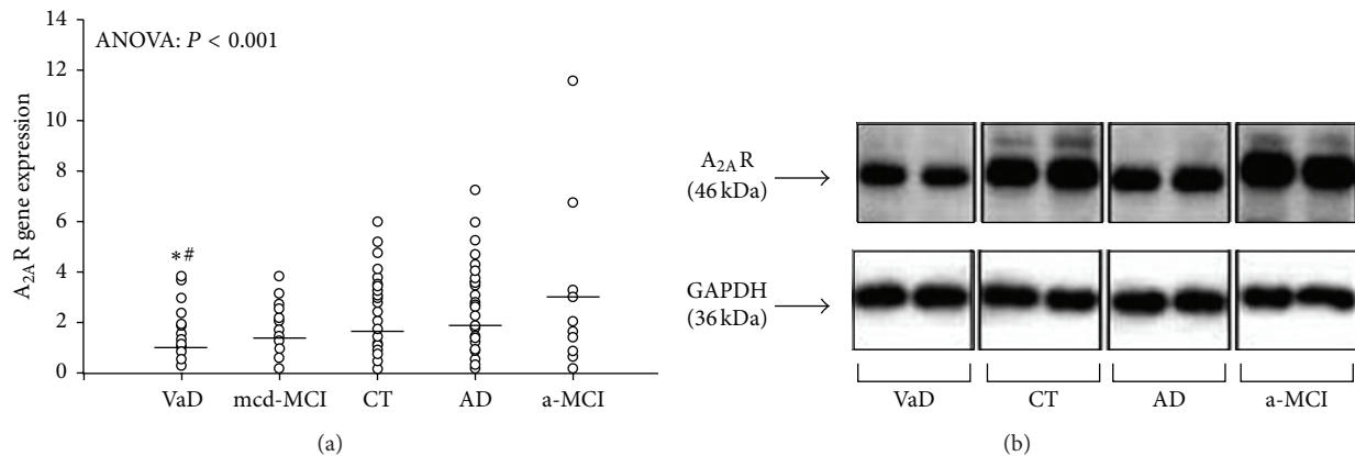
FIGURE 3: (a) Scatter plot of A 2A gene expression in PBMCs from VD, mcd-MCI, controls (CT), AD, and a-MCI subjects (the lines represent the mean value for each group). *P < 0.001 versus AD; #P < 0.05 versus a-MCI. (b) Representative picture of the western blot analysis of the A 2A densities in PBMCs extracts, running in duplicate, from one subject from the VD, CT, AD, and a-MCI groups, respectively.
