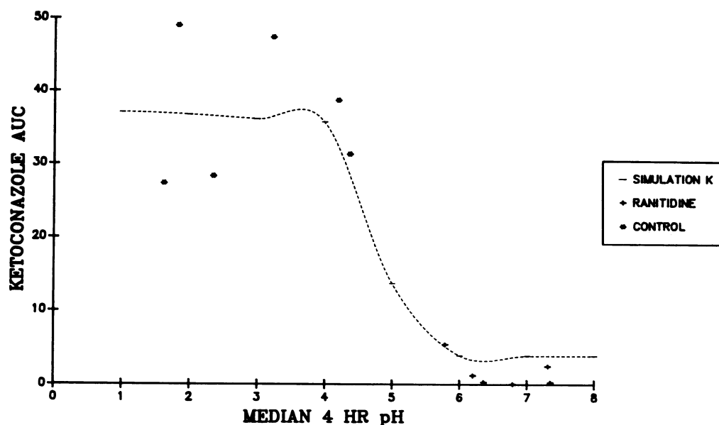
FIG. 3. Simulated ketoconazole bioavailability at different gastric pHs (---) based on in vitro dissolution data compared with actual patient data during control and ranitidine treatments.
