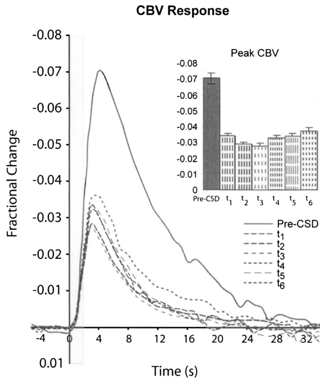
Fig. 2 Activity-related changes in CBV. CBV response to hindpaw stimulation produced a monophasic decrease in reflectance. Intensity time plots of pre- and post-CSD time points show a significant attenuation in response amplitude and duration following CSD. Shaded green region indicates stimulus duration. Inset shows the peak CBV values for pre- and post-CSD time points. Values reached a minimum at 20 to 30 min following CSD induction with only minimal recovery by 60 min. Error bars represent standard error.
