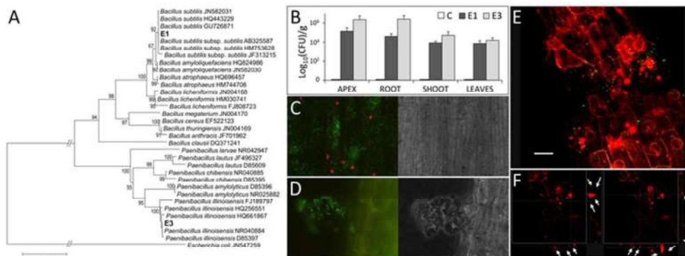
Figure 1. Phylogenetic affiliation of E1 ( B. subtilis ) and E3 ( P. illinoensis ), and rhizocompetence/colonization ability. (A) Phylogenetic trees of E1 and E3 using the complete 16SrRNA gene sequence. Neighbour-joining phylogenetic tree-based 16S rRNA gene sequences from E1 and E3, and their closest phylogenetic neighbours. Bootstrap values are indicated at nodes. Scale bar represents observed number of changes per nucleotide position. (B) Enumeration of Rif R versions of the E1Rif and E3Rif strains after isolation on selective medium. (C) Epifluorescence and phase contrast images of pepper roots densely colonized by E1-gfp. (D) Epifluorescence and phase contrast images of E1-gfp cells entrapping root hairs. (E) Confocal microscopy analysis of E1-gfp colonized roots. (F) The boxes indicated by dashed lines show orthogonal views of a three-dimensional confocal image created from a z-stack of x/y-scans. White arrows indicate the potential endophytic colonization of a root cortex by E1-gfp cells that were found in the orthogonal views of the inner root tissue.
