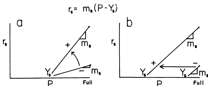
FIG. 1. Generalized formula for relating steady growth rate, r_s , to both turgor pressure, P , and to the action of auxin. a: Growth occurs only above a threshold turgor, Y_s , and increases above that threshold linearly with a slope of m_s . The action of auxin, to give high rate at full turgor, is to increase m_s while Y_s remains constant. b: The same relative increase in rate at full turgor is attained by lowering Y_s and leaving m_s constant. This diagram shows only extreme possibilities. Naturally auxin could affect both m_s and Y_s , and it is possible that rate is not linear with (P - Y_s) . To a rough approximation, the present experiments favor the model in a.
