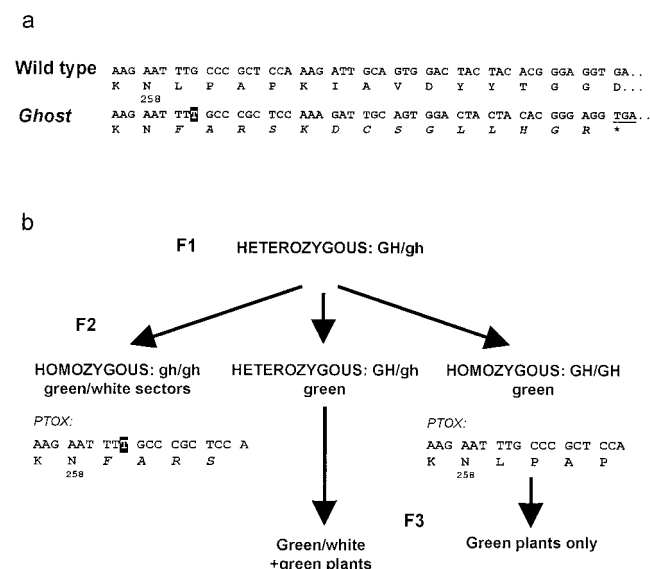
Figure 6. Identification of the tomato ghost gene. a , Partial sequence of the PTOX cDNA showing a T insertion (boxed) in ghost plants when compared to wild-type and deduced amino acid sequences. The amino acid sequence created by the mutation is shown in italics . b , Cosegregation of the ghost recessive phenotype and the mutation in the PTOX genomic sequence from a heterozygous F 1 plant to the F 2 generation. Homozygous F 2 wild-type plants were discriminated from heterozygous plants in the F 3 generation.
