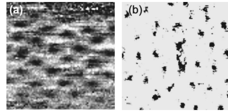
FIG. 37. 100×100 nm 2 STS images of (a) a slightly disordered oblique lattice in Y123 (from Maggio-Aprile et al. , 1995) and (b) a disordered vortex distribution in Bi2212 (from Hoogenboom et al. , 2001). Both images were acquired at T = 4.2 K and H = 6 T. The contrast is defined by the conductance measured at the gap energy (20 meV for Y123 and 30 meV for Bi2212) normalized by the zero-bias conductance.
