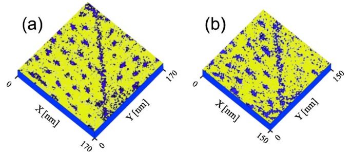
FIG. 39. (Color online) STS observation of a twin boundary in Y123. (a) 170 \times 170 \text{ nm}^2 image at H=3 \text{ T} ; the flux lines are distributed on both sides of the boundary with an equal density. (b) After reducing the field to 1.5 T, the flux lines pile up on the left domain and reach a density corresponding to about 2.5 T. From Maggio-Aprile et al. , 1997.
