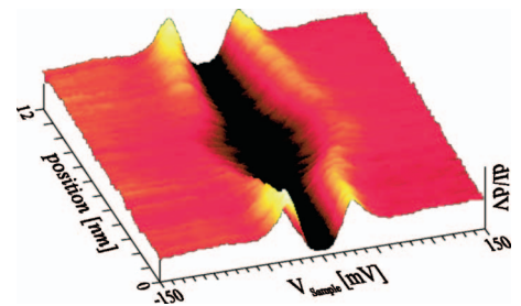
FIG. 46. (Color) Conductance spectra taken along a 12\text{-nm} path across a vortex core in overdoped Bi2212 ( T_c=77 \text{ K} ) at T=2.6 \text{ K} and H=6 \text{ T} . The spectra acquired at the center of the core reveal a pseudogaplike shape similar to the one observed above T_c . From Kugler, 2000.
