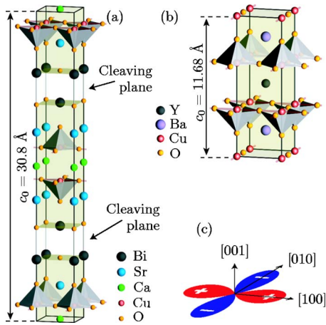
FIG. 5. (Color online) Crystal structure of the cuprate materials. (a) Tetragonal unit cell of \text{Bi}_2\text{Sr}_2\text{CaCu}_2\text{O}_{8+\delta} with a=b=5.4 Å defined along [110] and [\bar{1}10] , respectively. (b) Orthorhombic unit cell of \text{YBa}_2\text{Cu}_3\text{O}_{6+\delta} with a_0=3.82 Å along [100] and b_0=3.89 Å along [010] . (c) Schematics of the d_{x^2-y^2} superconducting gap in the unit-cell coordinate system. Note that a_0 and b_0 designate the lattice constants along the Cu-O-Cu bonds ( Pmmm space group for Y123), whereas a and b designate the lattice constants in larger unit cells ( Cmmm space group for Bi2212).
