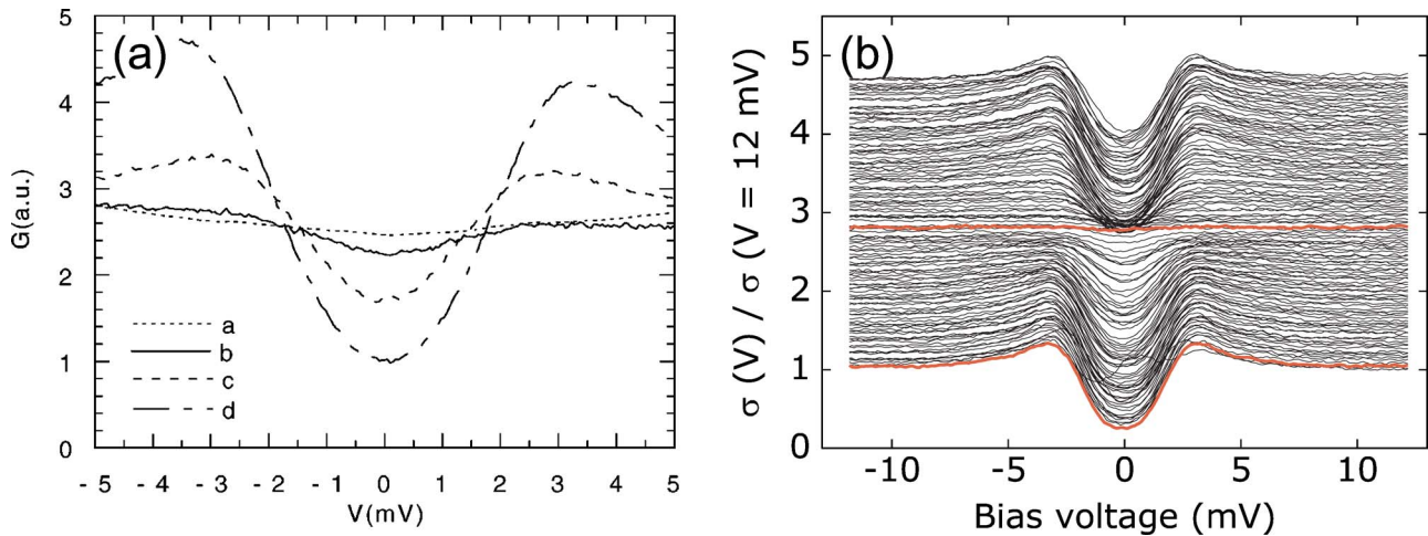
FIG. 43. (Color online) Examples of missing zero-bias peak in the vortex cores of conventional BCS superconductors. (a) Spectra acquired at 47 nm (dashed line) to the center of the core (dotted line) in \text{LuNi}_2\text{B}_2\text{C} at T=4.2 K and H=1.5 T. From DeWilde, Iavarone, Welp, Metlushko, Koshelev, Aranson, Crabtree, and Canfield, 1997. (b) 250-nm-long spectroscopic trace crossing a single vortex core in \text{MgB}_2 at T=2 K and H=0.2 T. From Eskildsen et al. , 2002.
