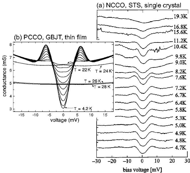
FIG. 28. Temperature evolution in electron-doped cuprates. (a) T dependence by STS of a \text{Nd}_{1.85}\text{Ce}_{0.15}\text{CuO}_4 single crystal (optimally doped, T_c = 20.5 K, \Delta_p \approx 4.5 meV). The tip is parallel to the [110] direction. From Hayashi, Ueda, et al. , 1998. (b) T dependence by grain-boundary junction tunneling (GBJT) on a \text{Pr}_{1.85}\text{Ce}_{0.15}\text{CuO}_4 thin film (optimally doped, T_c \approx 24 K, \Delta_p = 3.1 meV). Note that these junctions are of the SIS type and in plane. From Kleefisch et al. , 2001.
