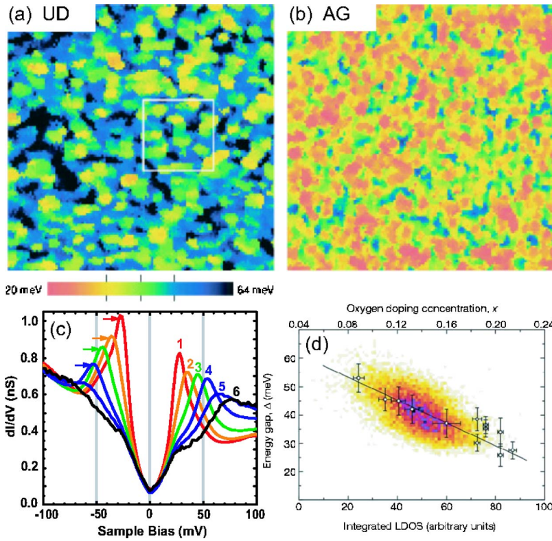
FIG. 16. (Color online) 56 \times 56 \text{ nm}^2 maps of the spatial gap distribution in (a) underdoped and (b) as-grown Bi2212 single crystals. Adapted from Lang et al. , 2002 . (c) Range of tunneling conductance spectra measured on inhomogeneous superconducting Bi2212. From McElroy, Lee, Hoffmann, et al. , 2005 . (d) Scatter plot of the superconducting gap versus the integrated local DOS in optimally doped Bi2212. From Pan et al. , 2001 .
