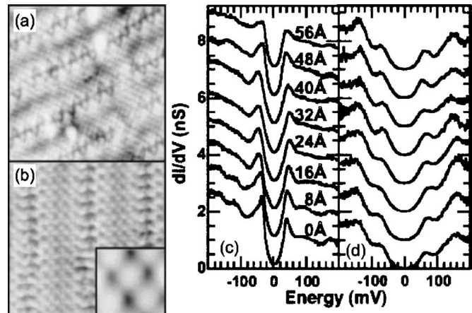
FIG. 7. STM topography and spectroscopy of a cleaved Bi 2 Sr 2 CaCu 2 O 8 thin film. (a) 10 \times 10 nm 2 topographic image of a BiO-terminated surface. (b) 6.4 \times 6.4 nm 2 topographic image of a CuO 2 -terminated surface (inset 0.8 \times 0.8 nm 2 ). Tunneling spectra taken at the indicated distances along a straight line (c) on the BiO plane and (d) on the CuO 2 plane. Spectra are offset for clarity, and all data were taken with V=200 mV and I=200 pA. From Misra et al. , 2002a.
