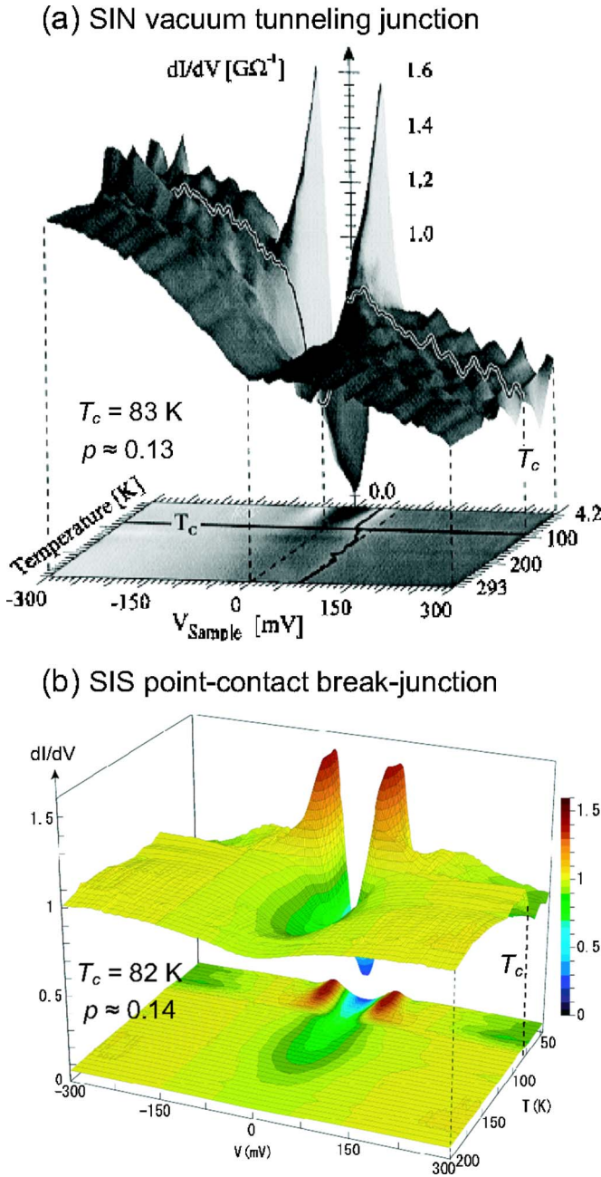
FIG. 25. (Color online) T dependence of the DOS of Bi2212 for two different junction types and tunneling techniques. (a) SIN vacuum tunneling using STM, T_c=83 \text{ K} , \Delta_p=44 \text{ meV} , T^* \approx 300 \text{ K} , and R_t=0.1\text{--}1 \text{ G}\Omega . From Renner, Revaz, Genoud, et al. , 1998. (b) SIS junction using PC-BJT, T_c=82 \text{ K} , \Delta_p \approx 27 \text{ meV} , T^* \approx 180 \text{ K} , and R_t=10\text{--}100 \text{ k}\Omega ; From Dipasupil et al. , 2002.
