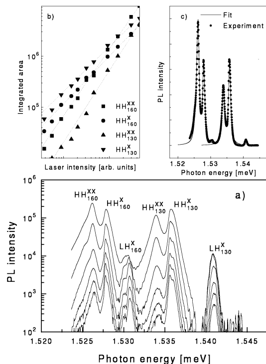
FIG. 2 Resonantly excited PL. (a) The photoluminescence spectra at different excitation densities, (b) linear increase of exciton luminescence and superlinear increase of biexciton luminescence with excitation density, and (c) fit of the photoluminescence lines with the inverted Boltzmann distribution.
