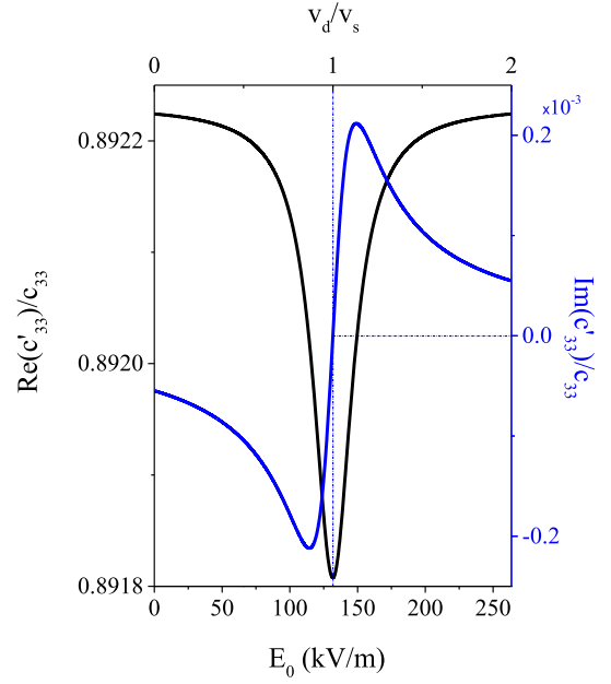
FIG. 2. c'_{33} is computed versus E_0 for ZnO with n = 10^4 n_i at \omega = 0.7 \omega_p . Top scale represents the data as a function of v_d/v_s . Left(right) axis represents the real(imaginary) part of c'_{33} . At the Cherenkov threshold, v_d = v_s (dash-dotted line at E_0 = 131.8 kV/m), the effective stiffness c'_{33} is purely real.
