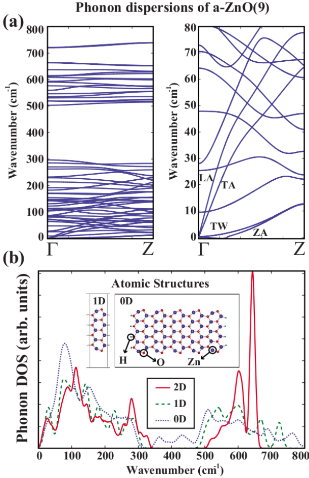
Figure 5: (Color online) (a) Phonon dispersion curves of a-ZnO(9) calculated by force constant method. Right panel presents the magnified view of the low lying modes. Here the well known out of plane, transverse and longitudinal acoustical modes are labeled, respectively, as ZA, TA and LA. The fourth acoustical twisting mode, which is indigenous to quasi 1D nanoribbons, is labeled as TW, because this mode corresponds to the twisting of the nanoribbon along the axis passing through the middle of the ribbon in the infinite direction. (b) Density of states (DOS) calculated for 2D planar ZnO (shown by solid lines); armchair a-ZnO(9) (shown by dashed lines); a finite size flake, i.e. a 5 unit cell long a-ZnO(9) (shown by dotted lines). The discrete frequencies due to finite size structure are gaussian broaden with \sigma=8 \text{ cm}^{-1} in order to compare with continuous DOS of 2D layer and quasi 1D ribbon. Quasi 1D (nanoribbon) and 0D (flake) honeycomb structures are shown by inset.
