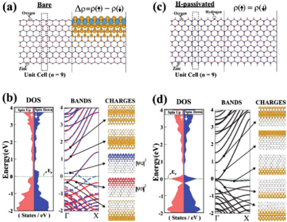
Figure 8: (Color online) Bare zigzag nanoribbon z-ZnO( n ) with n=9 : (a) Honeycomb structure with primitive unit cell delineated and difference charge density \Delta\rho of spin-up and spin-down states. (b) Total Density of spin-up and spin-down states (DOS), energy band structure and isosurface charge density of selected spin states. Large, medium and small filled balls indicate Zn, O and H atoms, respectively. (c) and (d) are same as (a) and (b). Yellow-light and blue-dark densities are for spin-up and spin-down states. Similarly red-continues and blue-dashed curves are spin-up and spin-down spin bands. Black lines are for nonmagnetic (spin-paired) bands.
