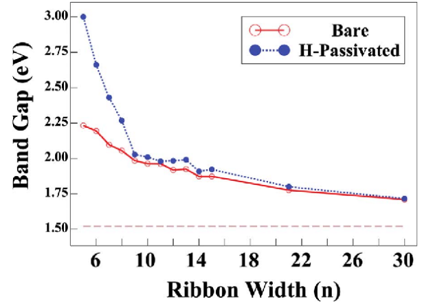
Figure 7: (Color online) Variation of the calculated band gaps of bare and hydrogen passivated ZnO armchair nanoribbons with their widths n . Dashed line indicates the band gap of the infinite 2D ZnO.
