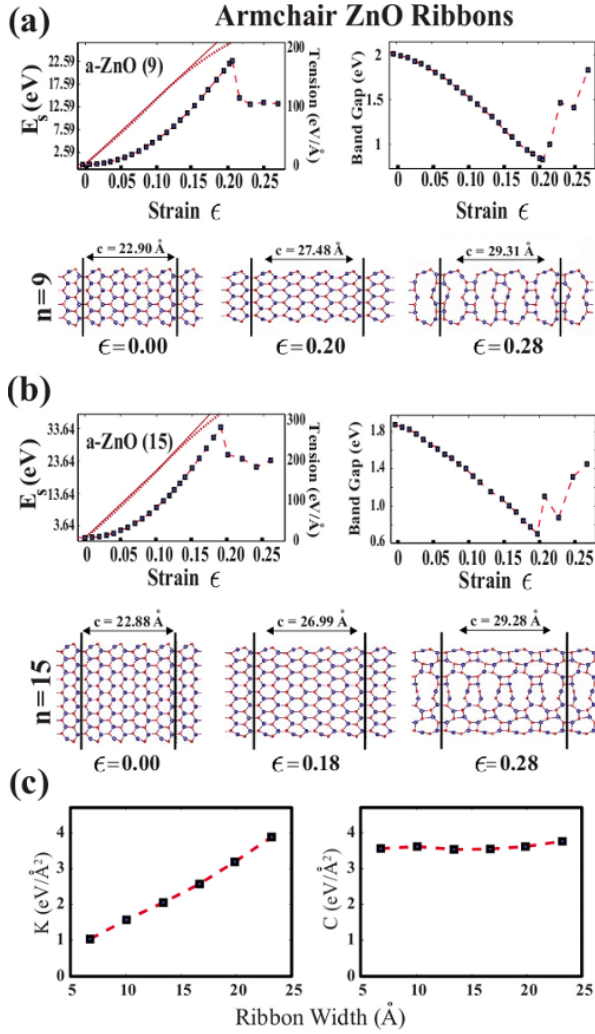
Figure 9: (Color online) (a) Variation of the strain energy E_s and band gap E_G of the bare a-ZnO( n ) ( n=9 ) with the applied uniaxial strain, \epsilon are shown by a curve with squares. Calculated tension shown by tin (red) curve is initially linear, but deviates from linearity for large \epsilon . Atomic structure for three different values of strain. The boundaries of the supercells comprising four unit cells and corresponding lattice constants c are indicated by vertical lines. (b) Same as (a) but for bare a-ZnO( n ) ( n=15 ). (c) Variation of force constant, \kappa and in-plane stiffness, C of a-ZnO with the width w of the nanoribbons.
