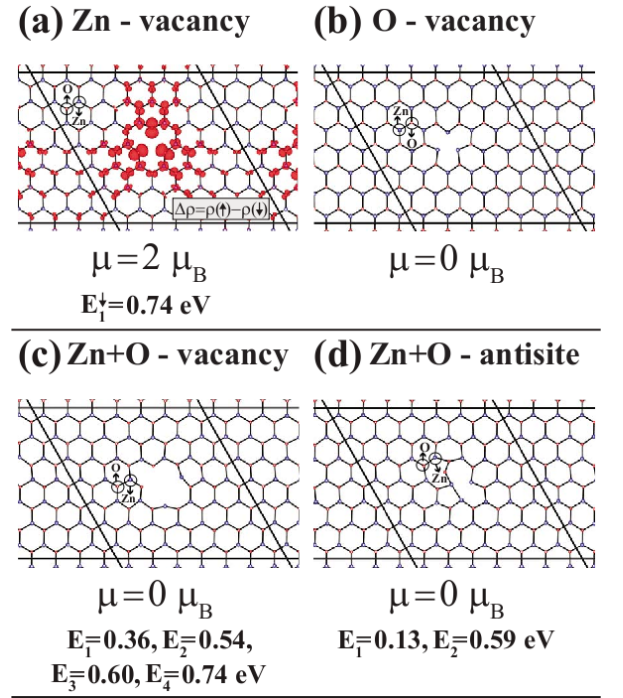
Figure 4: (Color online) Vacancy defects in a (7 \times 7) supercell of the monolayer of ZnO. (a) Relaxed atomic structure around the Zn-vacancy with isosurfaces of the difference charge density of spin-up and spin-down states, \Delta\rho = \rho(\uparrow) - \rho(\downarrow) . Energies E_i of localized states measured from the top of the valance band and the net magnetic moment per supercell in Bohr Magneton \mu_B . Blue-large and red-small balls indicate Zn and O atoms indicated by arrows. (b) O-vacancy. (c) Zn+O divacancy. (d) O+Zn antisite where neighboring O and Zn atoms are exchanged. The (7 \times 7) supercells each including one type of various vacancy defects are delineated by solid lines.
