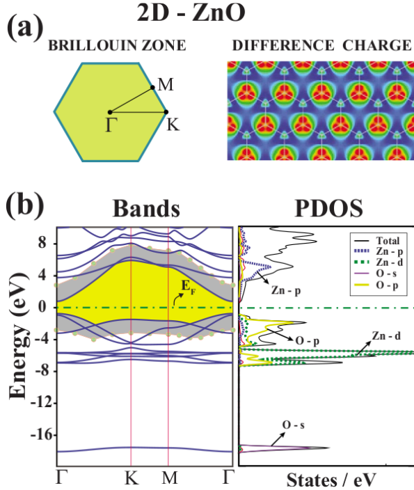
Figure 3: (Color online) Electronic structure of the 2D monolayer of ZnO. (a) Brillouin zone corresponding to 2D hexagonal lattice and difference charge density, \Delta\rho . (b) Energy band structure and density of states projected to the selected orbitals (PDOS) of constituent atoms. The band gap is shaded (painted in yellow) and the zero of energy is set at the Fermi level. Band edges corrected by GW_0 are indicated by small (light blue) circles. The band gap enlarged after GW_0 correction is shaded (painted light blue).
