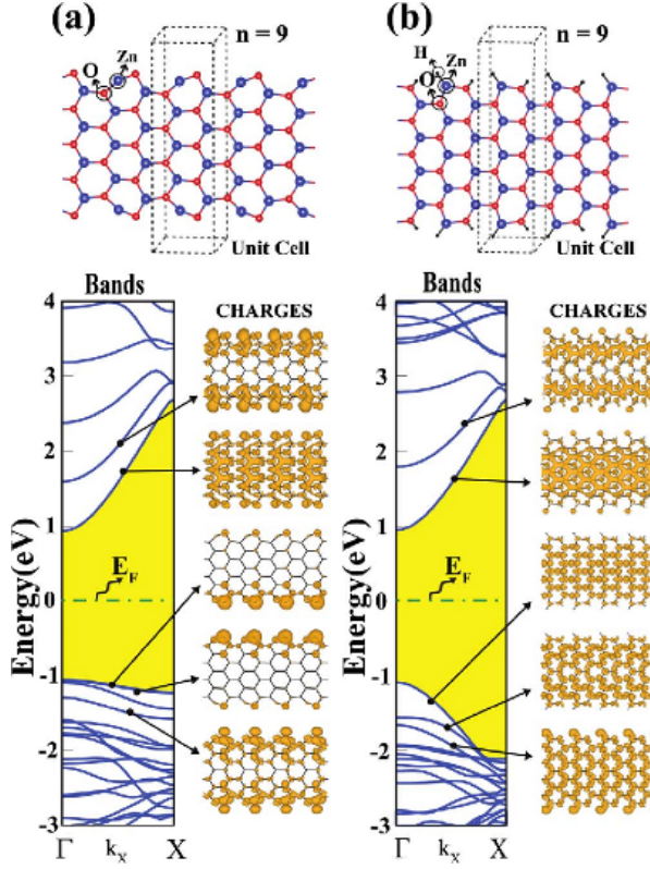
Figure 6: (Color online) Atomic and electronic structure of bare and hydrogen terminated armchair nanoribbons a-ZnO(9). (a) Atomic structure with unit cell comprising n=9 Zn-O atom pairs, energy band structure and charge density isosurfaces of selected states of bare nanoribbons. The charge of the bands of edge states are localized at the edge atoms. (b) Same as (a) but for hydrogen passivated nanoribbon. Large medium and small balls indicate Zn, O and H atoms, respectively. Unit cells are delineated by dashed lines.
