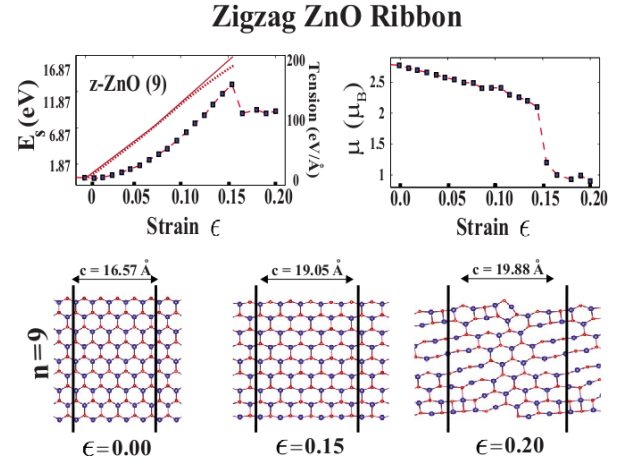
Figure 10: (Color online) Variation of the strain energy E_s , tension and magnetic moment \mu per supercell of the bare z-ZnO( n ) ( n=9 ) with the applied uniaxial strain. Atomic structures of the bare z-ZnO(9) for three different uniaxial strains. The supercells consist of five unit cells.
