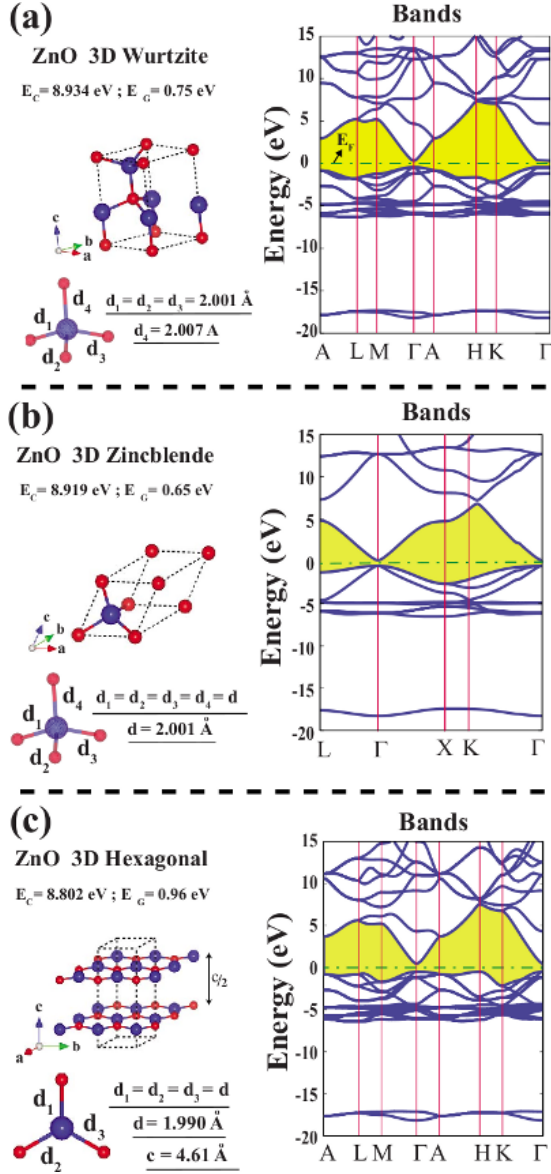
Figure 1: (Color online) Cohesive energies E_C per Zn-O pair, band gaps E_G , Zn-O bonds, atomic and energy band structures of 3D wurtzite (a), zincblende (b), and hexagonal (c) crystals of bulk ZnO. Red-small and blue-large balls correspond to O and Zn atoms, respectively. The gap between valence and conduction bands is shaded and the zero of energy is set at the Fermi level E_F . All structures including lattice constants are fully optimized.
