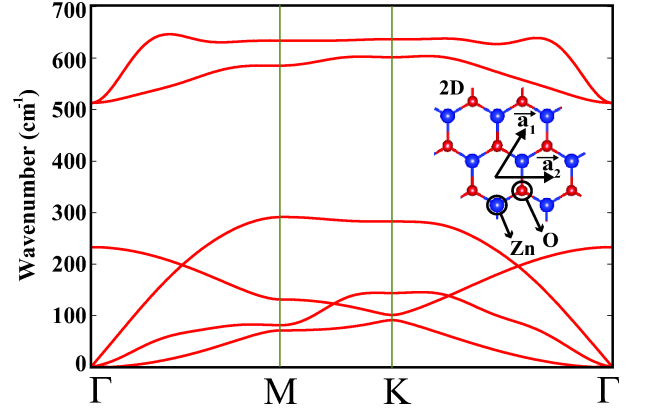
Figure 2: (Color online) Phonon dispersion curves calculated by force constant method for 2D monolayer ZnO. Atomic structure and hexagonal lattice vectors are shown by inset.
