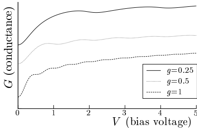
FIG. 4: At constant gate voltage: V_g L = \pi/2 , the period of oscillations is \pi/g t_L , i.e. depends strongly on the interaction strength. In order for this effect to be clearly visible, we scaled and shifted the functions differently, therefore the values of the G axes are not meaningful.
