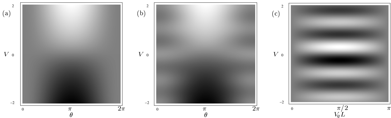
FIG. 5: Calculated spin for a nanotube with g = 0.25 , the component of the spin in the direction of the magnetization \vec{M}_1 as function of the angle between the two magnetizations \theta and the bias voltage V , at constant gate voltage (a) V_g = 0 and (b) V_g = \pi/2 ; and (c) the component of the spin perpendicular to the plane formed by the two magnetizations as a function of the gate and bias voltages.
