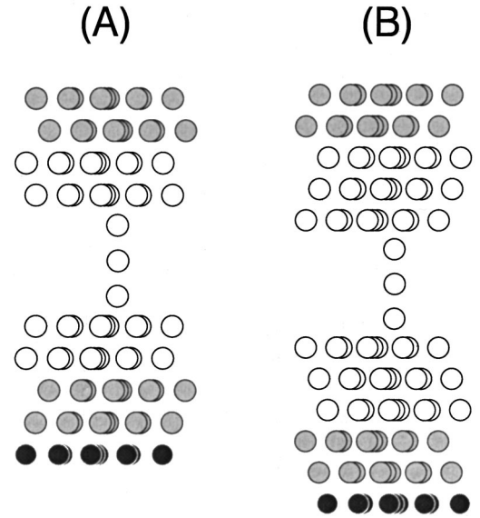
FIG. 8. Models used for the gold wires calculations. The white atoms correspond to contact region C while the gray atoms correspond to the L and R regions in Fig. 1. The black atoms are only included in the initial SIESTA calculation and can be added in order to yield a better initial density matrix for the subsequent TRANSIESTA run. We have used 2(A) and 3(B) surface layers in the contact region.
