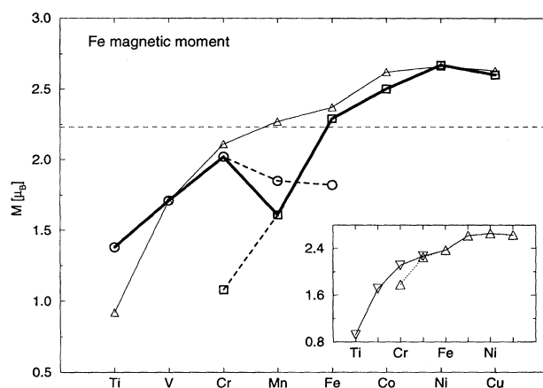
FIG. 2. Calculated magnetic moment of Fe at the interface with X . The bold solid line corresponds to the calculated ground-state moment for the monolayer situation. The broken lines indicate metastable solutions. Circles denote an AFM coupling and squares a FM coupling between the Fe and the overlayer X . The thin line (triangles) corresponds to the Fe interface moment for the bilayer situation. In the inset the Fe interface moment for the bilayer coverage is shown again. The broken line indicates the metastable solutions. Triangles pointing up indicate a FM coupling, triangles pointing down indicate an AFM coupling at the interface.
