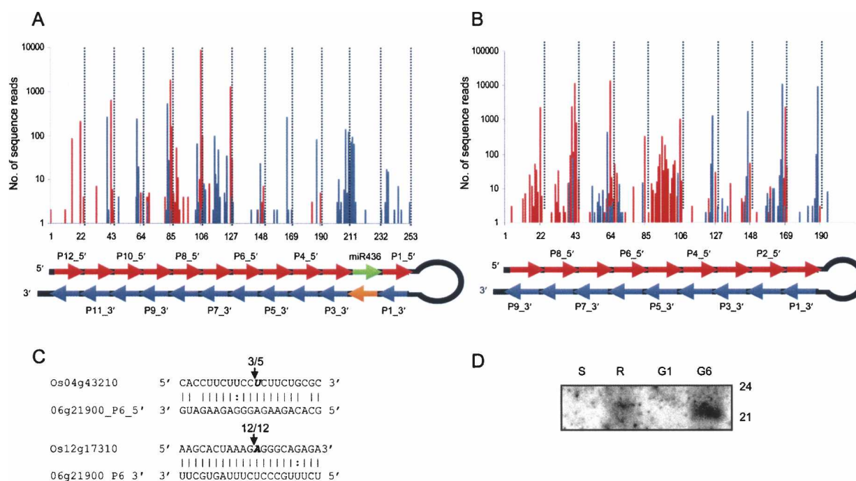
Figure 2. miRNA-like long hairpins producing phased 21-nt small RNAs. (A) Hairpin of the pre-miR436. In total, 13,141 and 2439 sequence reads were generated from the 5' and the 3' arms of the hairpin, respectively, and only 19 reads were mapped to the antisense strand. Of these sequences, 91.2% were 21 nt in length and 95.9% of these 21-nt small RNAs fell in phases of 21-nt spacing. The number of reads for all small RNAs with a common 5' terminus (regardless of size) is plotted, with red and blue bars representing sequences from the 5' and the 3' arms, respectively. The 21-nt phases corresponding to the 5' arm are indicated by the vertical dotted lines. Phase identifiers are shown above and below the hairpin. Nucleotide positions shown on the X-axis are based on the 5' arm of the hairpin starting from the 5' end of phase P12_5'. miR436 and miR436* are shown in green and orange, respectively. (B) A miRNA-like long hairpin generated from the antisense strand of LOC_Os06g21900. In total, 59,150 sequence reads were generated (~60% from the 5' arm and ~40% from the 3' arm; ~97% of the reads were from 6–10 DAF grains), including 97 reads mapped to the antisense strand; 54,857 (92.7%) reads were 21 nt in length and 93.9% of these 21-nt small RNAs were in exact 21-nt phases. The frequency and distribution of small RNAs is plotted as described in A. (C) 5' RACE validation of cleavage of predicted target mRNAs by P6_5' and P6_3'. (D) Expression of small RNAs from the newly identified long hairpin in different tissues detected by a probe antisense to the 3' arm of the hairpin (218 nt in length). The blot used was the same as that for miR1861 shown in Figure 1C. (S) Shoots; (R) roots; (G1) 1–5 DAF grains; (G6) 6–10 DAF grains.
