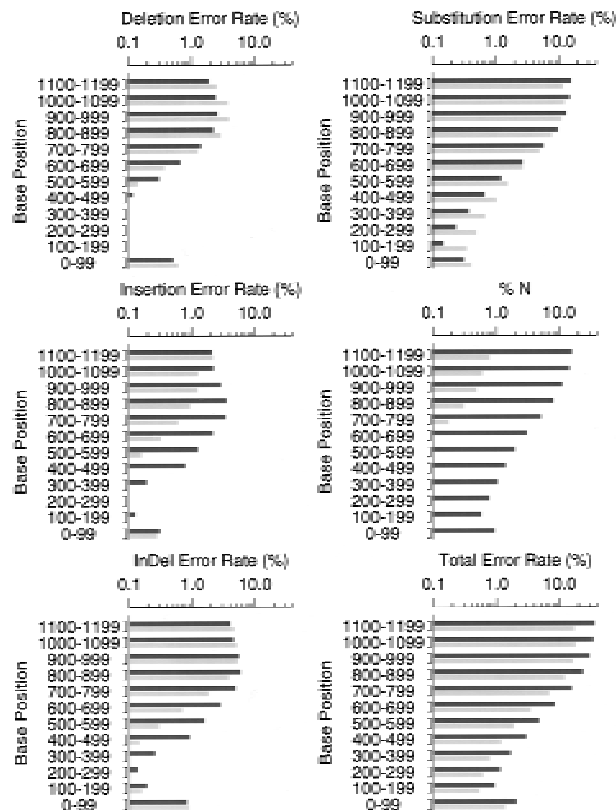
Figure 3 Phred (gray bars) and ABI (black bars) error rates for dye primer data in cosmid set 3.
