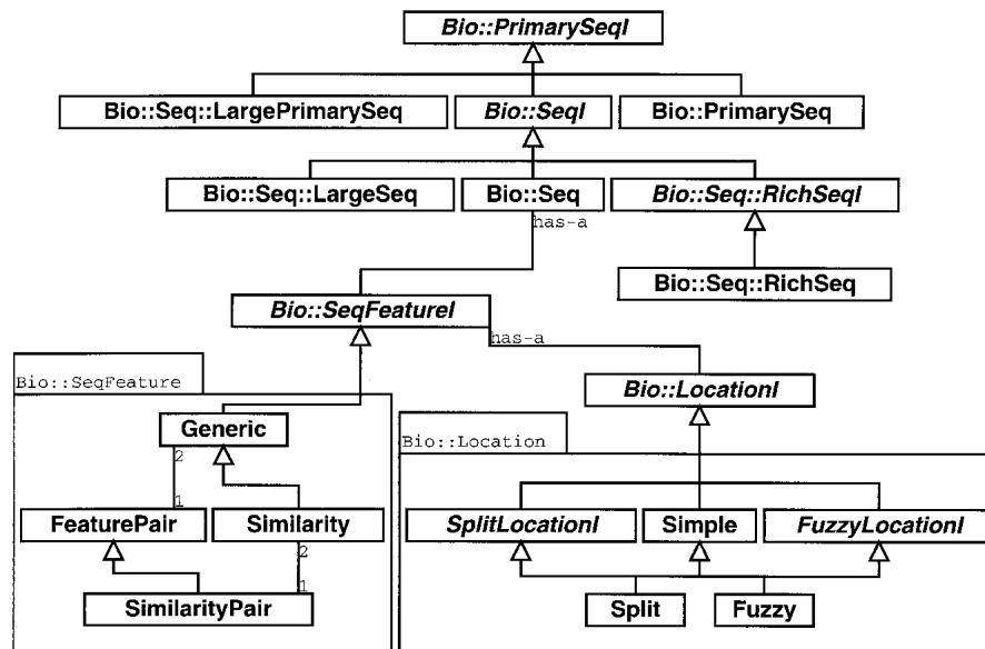
Figure 2 This figure shows a portion of the Bioperl object model including the interfaces (shown in italicized type) for sequences (PrimarySeq, SeqI, RichSeqI) and their implementations PrimarySeq (general sequence), Seq (sequence with features), RichSeq (sequence with features and rich annotation), LargePrimarySeq (for sequences too large to be held in a program's memory), and LargeSeq (large sequences with features). Also included in the diagram is the sequence feature interface (SeqFeatureI) and its implementations Similarity (manage similarity information), FeaturePair (paired feature information), and SimilarityPair (paired similarity information such as a pair-wise alignment information). Additionally, the diagram shows the location objects that manage Simple (start, end, and strand information), Split (multiple start and end spots on a sequence such as a set of exons), and so-called Fuzzy locations (where start, end or span is not exact) for sequence features.
