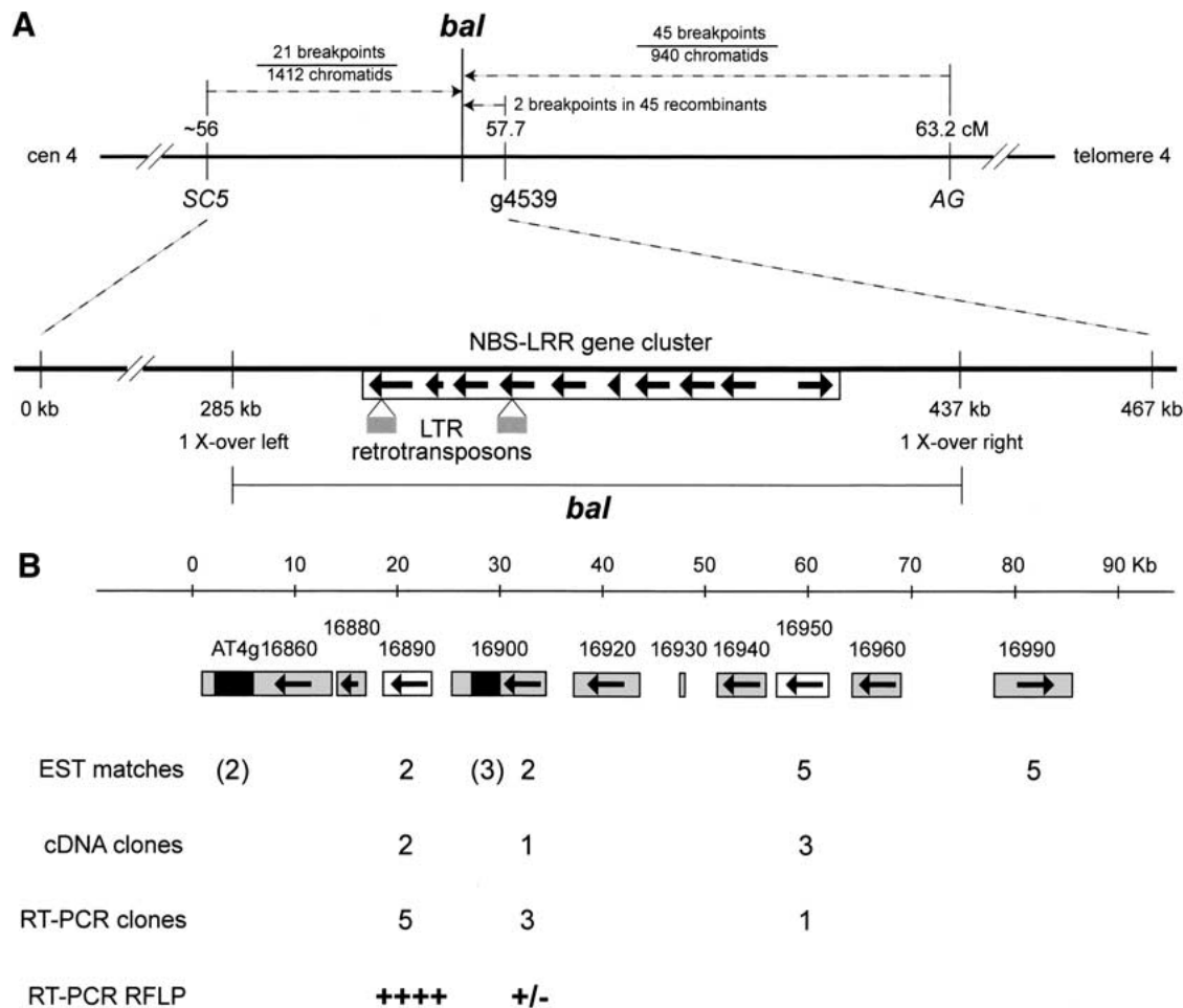
Figure 5. Map-based identification of the BAL locus. (A) (top) A genetic map of the region carrying the bal alteration. Distances are marked in centiMorgans (cM), and relevant genetic markers are shown beneath the genetic map. The dashed lines above the genetic map indicate the distribution of recombination breakpoints in the region. (Bottom) A physical map of the region with the minimal genetic window containing the bal alteration shown by the bracketed line. The 90-kb NBS-LRR gene cluster ( RPP5 -like) from strain Columbia is shown, as well as the positions of two LTR retrotransposons. (B) A higher resolution representation of the predicted RPP5 -like genes (white and gray boxes) and LTR retrotransposons (filled boxes) in the 90-kb NBS-LRR gene cluster. Arrows indicate the predicted direction of transcription. Gray boxes indicate RPP5 -like genes that are predicted to be nonfunctional because of point mutations and/or retrotransposon insertions. White boxes indicate genes predicted to encode functional NBS-LRR-class proteins. The results of our gene expression survey of the region are shown below the physical map. The number of matches in the public EST databases is indicated below each predicted coding sequence and the LTR retrotransposons (in parentheses). The number of matches to six newly isolated cDNA clones from the region is also shown. The distribution of sequenced RT-PCR clones and RFLP analysis of RT-PCR bulked products (data not shown) indicates that At4g16890 is the predominantly expressed gene in the cluster. Noël et al. (1999) use an alternative nomenclature to describe this region: At4g16890 = RPP5 homolog Col-B .
